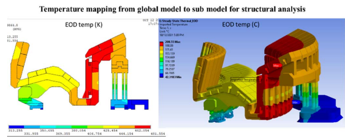
Fig. 10. Mapping temperature from 2-D global model to 3-D structural model.
