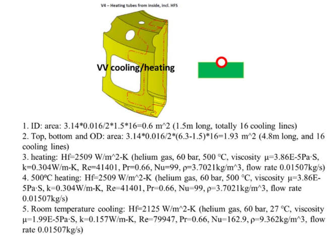
Fig. 6. Calculating the parameters of helium gas heating/cooling of VV.
