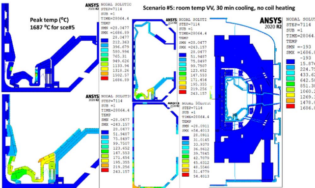
Fig. 7. Peak temperature (°C) and end-of-16th-pulse (EOP) temperature distributions.
