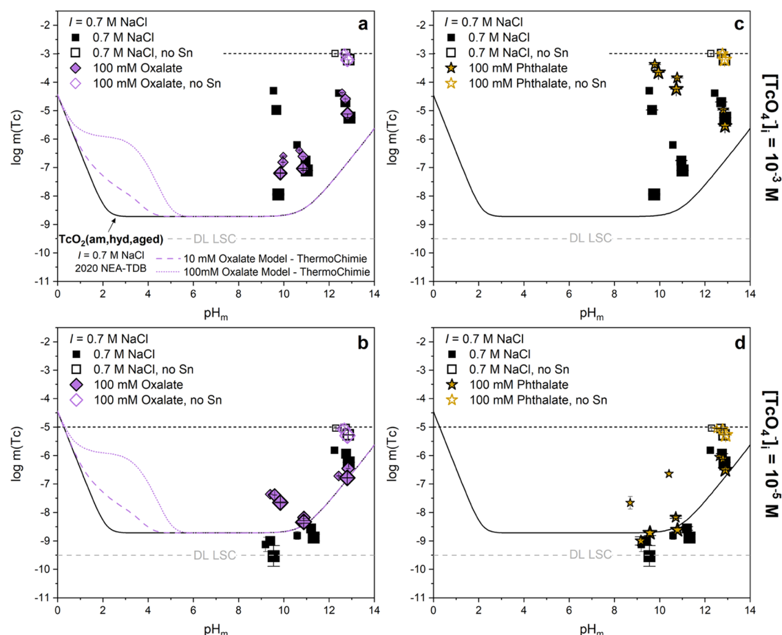
Figure 3. Oversaturation experimentally measured aqueous m(\text{Tc})_{\text{tot}} at [L]_{\text{tot}} = 0 \text{ M} (black squares) or 100 \text{ mM} (colored symbols) in the presence (solid symbols) or absence (open symbols) of \text{SnCl}_2 with [\text{TcO}_4^-]_i = 10^{-3} \text{ M} (top panel) or 10^{-5} \text{ M} (bottom panel) where L = (\text{a, b}) oxalate and (\text{c, d}) phthalate. Data points increase in size with increasing equilibration time: t_1 = 41 days, t_2 = 88 days, and t_3 = 173 days. Solid and dotted lines correspond to the thermodynamically calculated solubility of \text{TcO}_2(\text{am,hyd}) under different solution conditions based on values from the literature (Table S3). 9,10,15–17 Gray dashed lines represent the LSC detection limits for the experimental analyses, and all error bars are either represented or contained within data symbols.
