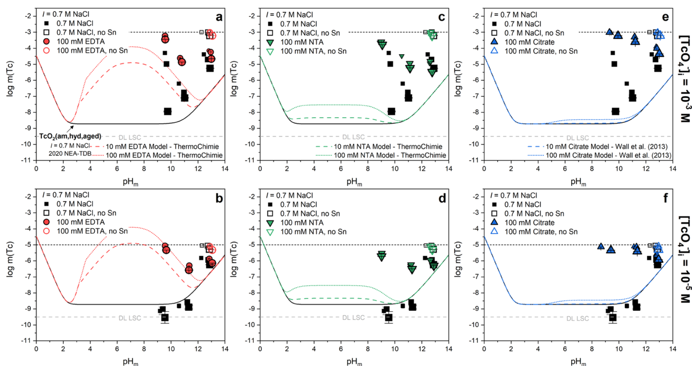
Figure 4. Oversaturation experimentally measured aqueous m(\text{Tc})_{\text{tot}} at [L]_{\text{tot}} = 0 M (black squares) or 100 mM (colored symbols) in the presence (solid symbols) or absence (open symbols) of \text{SnCl}_2 with [\text{TcO}_4^-]_i = 10^{-3} M (top panel) or 10^{-5} M (bottom panel) where L = (a, b) EDTA, (c, d) NTA, and (e, f) citrate. Data points increase in size with increasing equilibration time: t_1 = 41 days, t_2 = 88 days, and t_3 = 173 days. Solid and dotted lines correspond to the thermodynamically calculated solubility of \text{TcO}_2(\text{am,hyd}) under different solution conditions based on values from the literature (Table S3). 9,10,15–17 Gray dashed lines represent the LSC detection limits for the experimental analyses, and all error bars are either represented or contained within data symbols.
