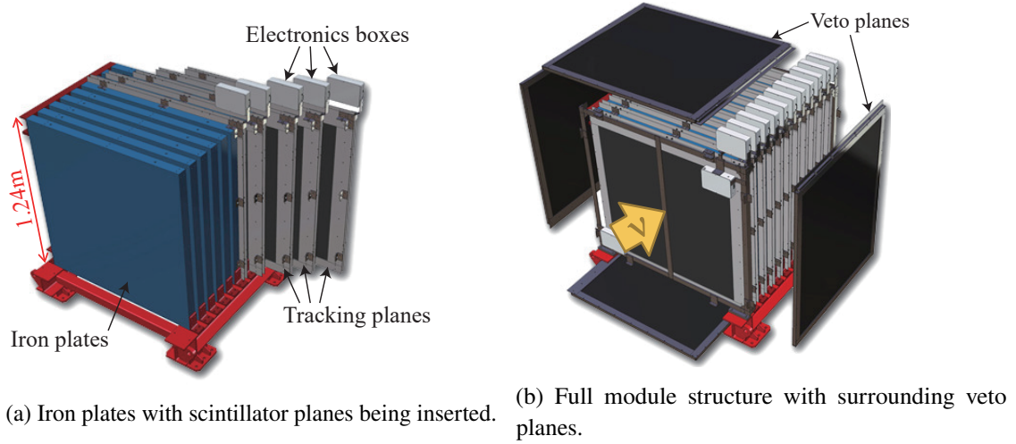
Figure 7. Structure of an INGRID module. Scintillator tracking planes are interleaved with iron plates (a). The sides of the module are then surrounded by scintillator veto planes (b).
