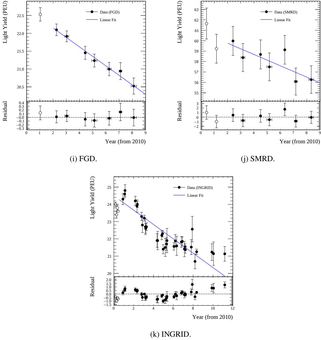
Figure 13. Light yield change in each subsystem (upper pad) and residual when the linear fit result is subtracted from each data point (lower pad), for T2K Runs 3–9 (ND280) and Runs 2–11 (INGRID). The x-error bars (time) show the standard deviation in the hit times for each data aggregation period, and the y-error bars (light yield) show the quadratic sum of the light yield stability uncertainty and the uncertainty on the ND280 Landau-Gaussian MIP MPV or INGRID MOM. Hollow data points are excluded from the fits as the current calibration procedures and cosmic ray triggering prescale were not finalised at that time. The exponential fits used in section 5 are not shown as the linear and exponential fit lines for all detectors overlap almost completely on the displayed timescales.
