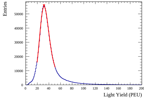
Figure 10. Example MIP light yield distribution in ECal Barrel X after calibrations and corrections are applied. The MIP most probable value (MPV) in Pixel Equivalent Units (PEU) is extracted from a Landau-Gaussian fit to the distribution. A PEU corresponds to the signal of a single MPPC pixel.
