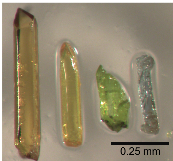
Figure 1. An image of single crystals of (left to right) \text{LaBS}_3 , \text{CeBS}_3 , \text{PrBS}_3 , and \text{NdBS}_3 .
