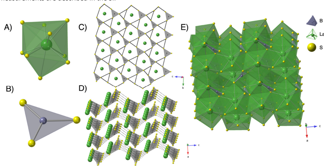
Figure 2. A schematic of the \text{LnBS}_3 structure showing the (A) \text{LnS}_9 and (B) \text{BS}_3 building blocks as well as an (C) illustration of the corrugated kagome nets, (D) how they stack within the structure, and (E) an image of the overall crystal structure.
