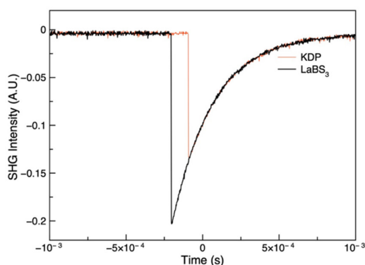
Figure 3. Powder SHG data of a sample of \text{LaBS}_3 compared to a standard sample of KDP with a particle size between 90–125 \mu\text{m} .
