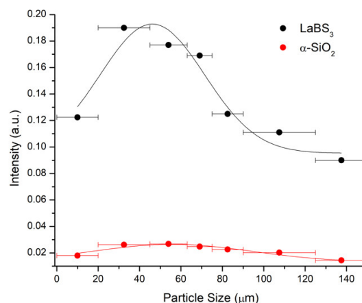
Figure 4. Powder SHG phase-matching experiment on \text{LaBS}_3 compared to a standard \alpha\text{-SiO}_2 with particle size ranges of <20, 20–45, 45–63, 63–75, 75–90, 90–125, and 125–150 \mu\text{m} . The lines are not fits to data, but to guide the eye.
