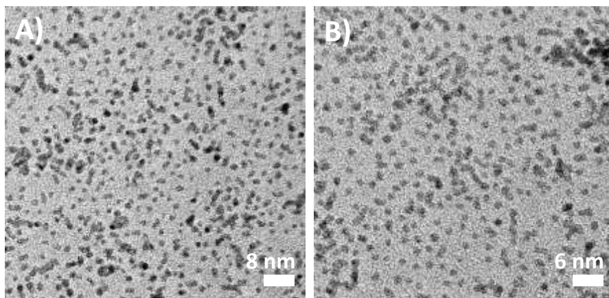
Figure 2. TEM micrographs at different magnification of Ir NPs obtained from 100 mM \text{IrCl}_3 in 1 M NaOH in methanol at 60\text{ }^{\circ}\text{C} for a week for a total volume of 0.2 mL. See also Figure S5-S6.
