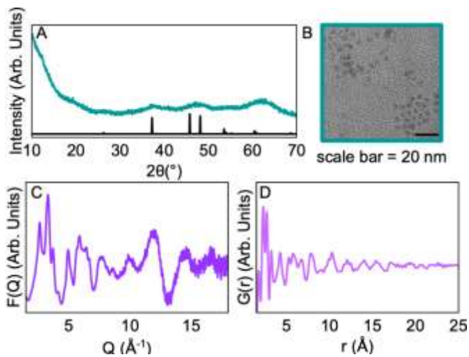
Figure 3. Characterisation of Cu 2-x S NPs obtained in an NMR tube setup. (A) Using a lab-source XRD instrument (blue) compared to a calculated diffraction pattern of \beta -chalcocite taking the space group P6 3 /mmc (black). (B) TEM micrographs of the washed NPs. Scale bar is 20 nm. (C) Displays of the F(Q) and (D) PDF (G(r)) of X-ray total scattering data collected at Argonne national lab at beamline 11-ID-B.
