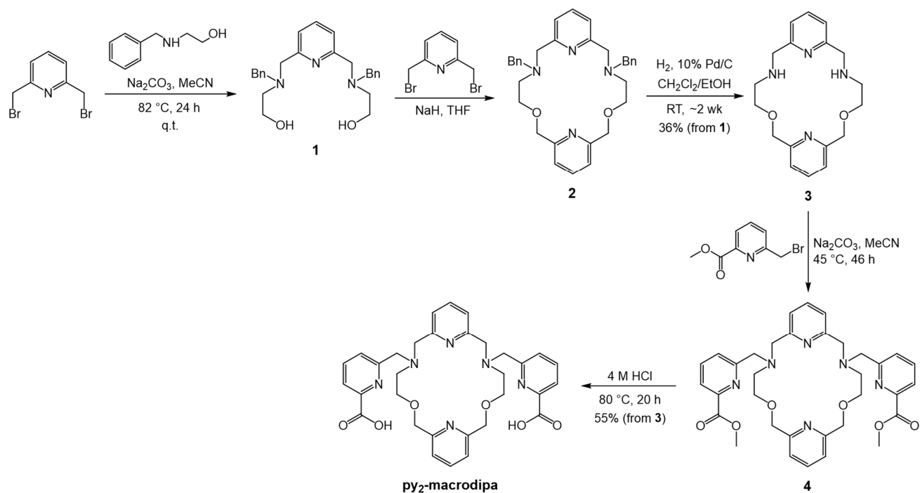
Scheme 2. Synthetic Route to py 2 -macrodipa.
