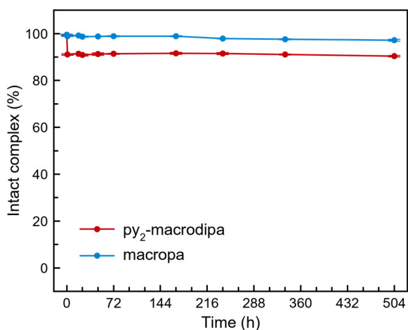
Figure 6. The stability of [ 225 Ac]Ac 3+ -py 2 -macrodipa and [ 225 Ac]Ac 3+ -macropa in human serum at 37 °C.
