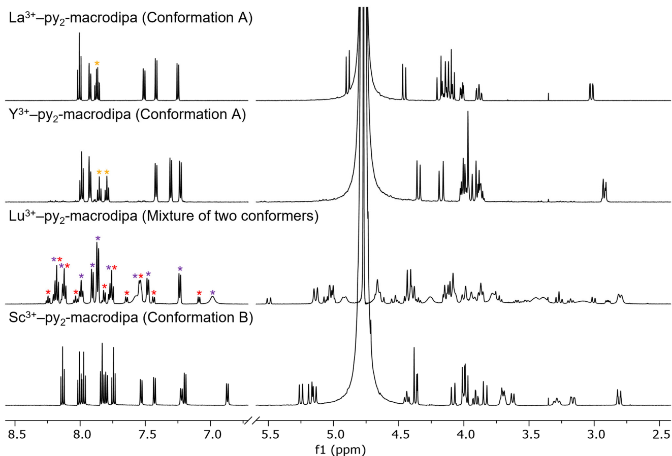
Figure 2. ^1\text{H} NMR spectra of \text{La}^{3+} -, \text{Y}^{3+} -, \text{Lu}^{3+} -, and \text{Sc}^{3+} - \text{py}_2 -macrodipa complexes (600 MHz, \text{D}_2\text{O} , pD 7, 25 °C). The yellow asterisks in the spectra of the \text{La}^{3+} and \text{Y}^{3+} complexes highlight the decrease in symmetry of Conformation A in moving from larger to smaller ions. The purple (Conformation A) and red (Conformation B) asterisks in the spectrum of the \text{Lu}^{3+} complex indicate the two conformers present in solution.
