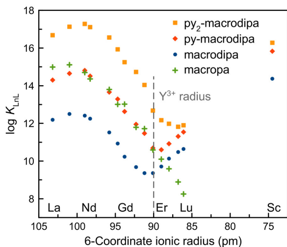
Figure 4. Stability constants of \text{Ln}^{3+} complexes formed with \text{py}_2 -macrodiapa, \text{py} -macrodiapa, macrodiapa, and macropa plotted versus ionic radii.
