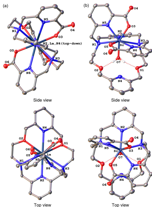
Figure 1. Crystal structures of (a) [La(py_2\text{-macrodipa})]^+ and (b) [Sc(py_2\text{-macrodipa})(OH_2)]^+ complexes. Thermal ellipsoids are drawn at the 50% probability level. Solvent, counterions, and nonacidic hydrogen atoms are omitted for clarity.
