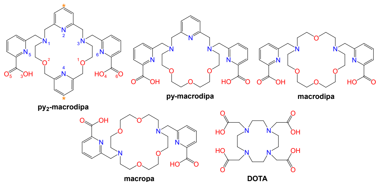
Chart 1. Structures of Ligands Discussed in This Work.
