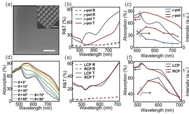
Fig. 3. Experimentally measured optical spectra. (a) SEM images of the MAPbI 3 metasurface; the scale bar indicates 5 \mu m. Inset: SEM image tilted at 30°; the scale bar indicates 500 nm. (b), (e) Reflection and transmission spectra under (b) incident LP light [line description is the same as in Fig. 1(b)] and (e) CP light [line description is the same as in Fig. 1(d)]. (c), (f) Absorption and PLE spectra under (c) incident LP light ( x -polarization, lower solid curve; y -polarization, upper solid curve) and (f) CP light (LCP, upper solid curve; RCP, lower solid curve). (d) The absorption of LP light with different polarization angles (from top to bottom, 90°, 75°, 60°, 45°, 30°, 15°, 0°).
