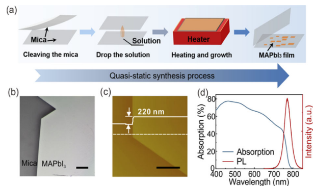
Fig. 2. HOIP ( \text{MAPbI}_3 ) films. (a) Schematic of the quasi-static solution growth process. (b) Optical microscopy image. (c) AFM image. (d) Absorption (left curve) and PL (right curve) spectra. The scale bars indicate 10 \mu\text{m} .
