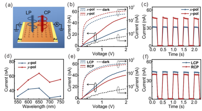
Fig. 4. Electrical characteristics of the metasurface. (a) Measurement setup used for the electrical measurements. (b), (e) Measured I – V curves under (b) LP light illumination ( x -polarization, lower dashed curve; y -polarization, upper dashed curve) and (e) CP light illumination (LCP, upper dashed curve; RCP, lower dashed curve). The data associated with the left axis are I_{\text{light}} - I_{\text{dark}} values on a linear scale, and the data associated with the right axis are values of the currents I_{\text{light}} and I_{\text{dark}} on a logarithmic scale. (c), (f) Time-resolved photocurrents of the device under (c) periodic on/off LP light illumination ( x -polarization, lower curve; y -polarization, upper curve) and (f) CP light illumination (LCP, upper curve; RCP, lower curve). (d) Measured photocurrents of the metasurface with incident LP light of different excitation wavelengths ( x -polarization, lower solid curve; y -polarization, upper solid curve).
