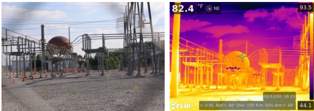
Fig. 6: Visible and IR photographs of a section of the electrical substation.
