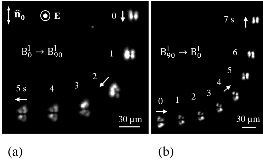
Fig.7. Electric field controls symmetry, mutual transformations, and direction of propagation of low-frequency directrons. (a) B_0^1 transforms into B_{90}^1 and changes the direction of propagation after the voltage is raised at t=0 s from 8 V to 11 V. (b) B_{90}^1 transform into B_0^1 when the voltage at t=0 s is decreased from 11 V to 8 V. CCN-47 doped with 0.005wt% of TBABr. Redrawn from Li et al. [46].
