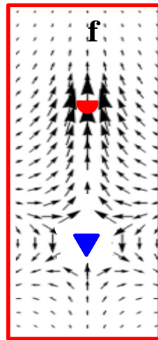
Fig.21. In-plane shifts of +1/2 defects upon heating. (a) PolScope image of a flat LCE coating at 23\text{ }^{\circ}\text{C} with periodic lattice of defects of strength \pm 1/2 ; red boxes A and blue boxes B enclose two types of pairs: in pair A, the director \hat{\mathbf{n}}(\mathbf{r}) is perpendicular to the line connecting the two cores, in pair B, \hat{\mathbf{n}}(\mathbf{r}) connects the cores. (b) Separation distance between +1/2 and -1/2 cores increases in pairs A and decreases in pairs B as the temperature increases. (c) Director configuration and active force \mathbf{f}(\mathbf{r}) calculated using Eq.(11) for pair A. (d) The same for pair B. Redrawn from Babakhanova et al. [226].
