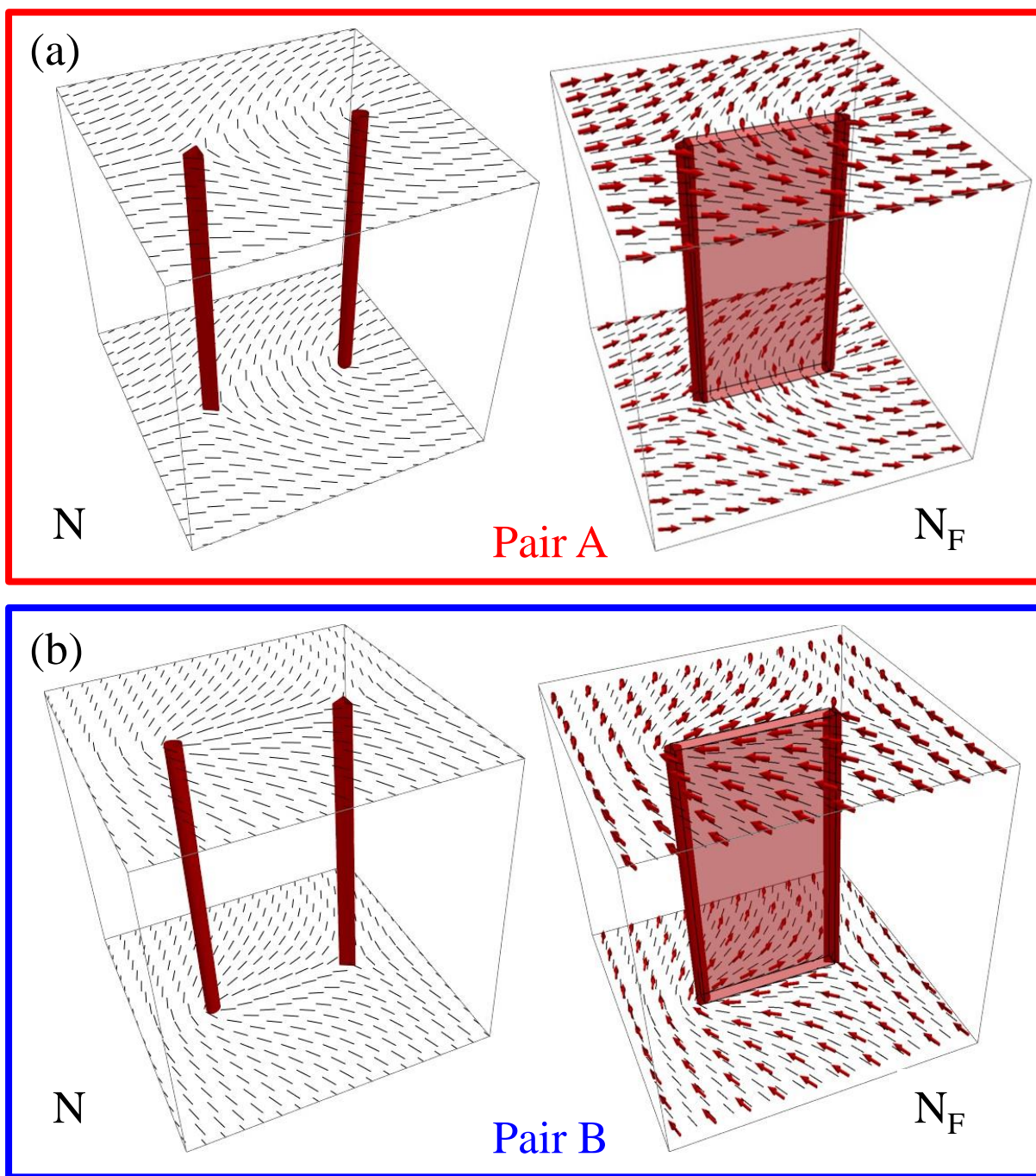
Fig.37. Pairs of \pm 1/2 disclinations of type A (a) and type B (b) in a nematic serve as seeds of domain walls in the ferroelectric nematic N_F . Redrawn from Lavrentovich [564].
