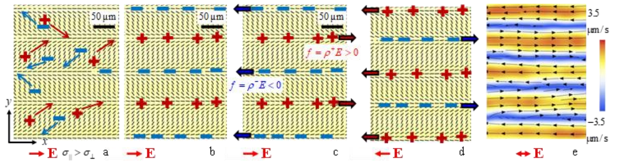
Fig.15. LCEO in a nematic electrolyte with a pre-designed director. Ticks represent local director visualized by PolScope: (a) the electric field \mathbf{E} drives “+” and “-” electric charges along the x-axis but because of the anisotropic conductivity, the charges shift also along the y-axis, (b) creating separated lanes of space charges; (c) the electric field moves them along the x-axis; (d) reversal of the field changes polarity of charges but does not change the Coulomb force; (e) an AC field of frequency 5 Hz creates lanes of LCEO flows of alternating direction. Redrawn from Peng et al. [187].
