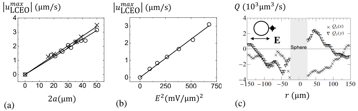
Fig.12. Quantitative parameters of LCEO around a glass sphere in a uniform AC electric field of frequency 5 Hz. (a) Maximum LCEO velocity around tangentially anchored (circles) and perpendicularly anchored (crosses) spheres increases linearly with the diameter 2a of the sphere; velocity patterns are of quadrupolar symmetry in both cases; E = 26 \text{ mV}/\mu\text{m} . (b) Maximum LCEO velocity around a tangentially anchored sphere of diameter 2a = 50 \mu\text{m} grows as E^2 . (c) Volume of the LC flow around a sphere with perpendicular anchoring and a dipolar structure (diameter 50 \mu\text{m} ), shown in Fig.10i, passing along the x –axis and along the y – axis defined in Fig.10. The nematic is pumped from right to left. Modified from Lazo et al. [175].
