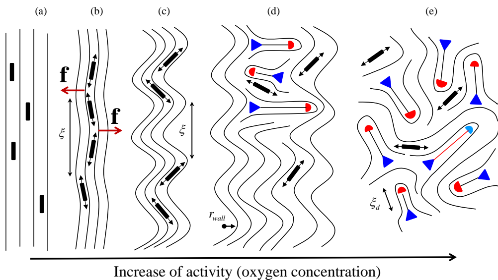
Fig. 28. Development of nonequilibrium regimes in a living liquid crystal, following the experimental data by Zhou et al. [276]: (a) equilibrium state, dormant bacteria; (b,c) bend instability, with the period \xi decreasing as activity increases; hydrodynamic interaction of bacteria in close proximity to each other produces an active force \mathbf{f} that enhances a fluctuative bend; (d) nucleation of m = \pm 1/2 disclination pairs of the B-type, see Fig.21d; +1/2 cores move away from -1/2 cores; (e) topological turbulence. Swimming bacteria of pusher type are shown as rods with two arrows.
