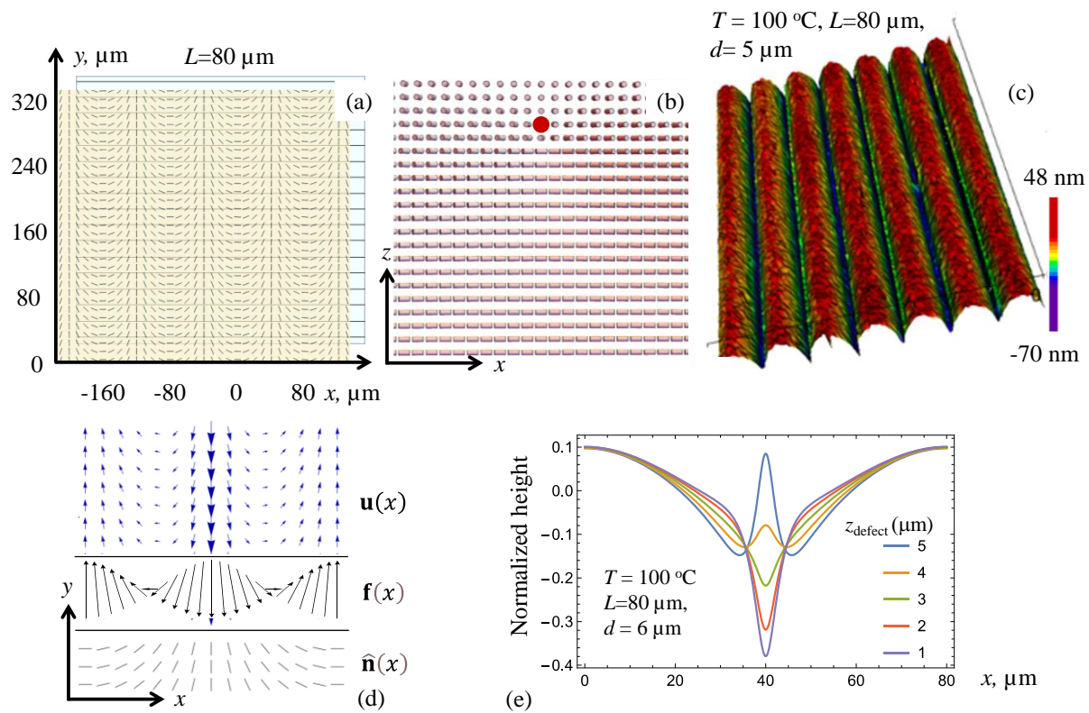
Fig.22. LCE coating with a prepatterned system of singular disclinations. (a) Director patterns on the top and bottom surfaces. (b) Vertical cross-section of unpolymerized nematic with the core of the disclination shifted towards the patterned surface. (c) Surface profile of LCE coating of thickness d = 5 \mu\text{m} and period L = 80 \mu\text{m} at the elevated temperature. (d) Linear elasticity theory calculations of in-plane displacements \mathbf{u}(x) of the heat-activated coating and the activation force \mathbf{f}(x) for the corresponding director field \hat{\mathbf{n}}(x) . (e) Linear elasticity theory calculations of the out-of-plane displacements of the heat-activated LCE coating ( d = 6 \mu\text{m} , L = 80 \mu\text{m} ) for different locations of the disclination line in the LCE bulk; the top free surface of the coating is patterned as shown in part (a). Redrawn from Babakhanova et al. [265].
