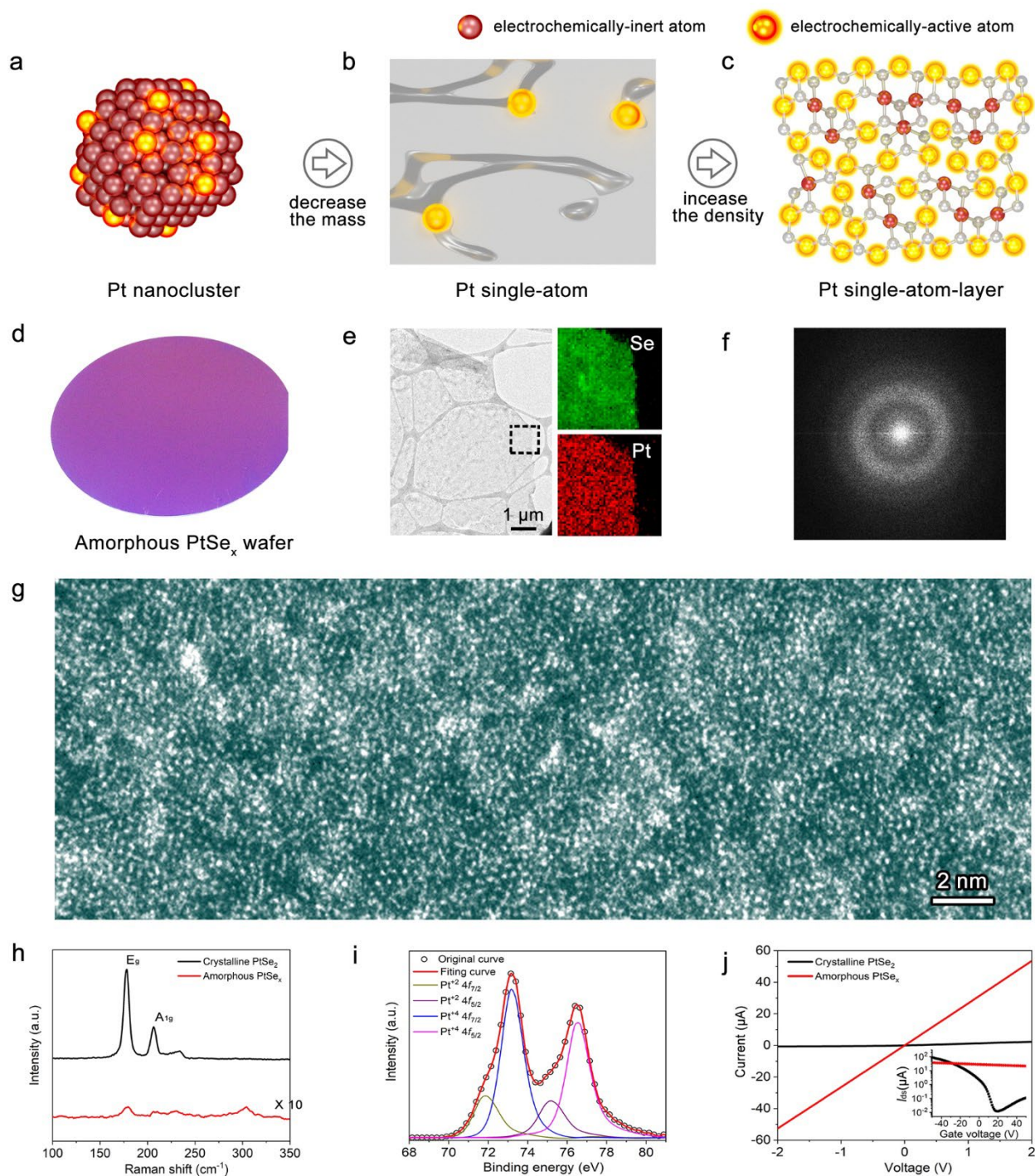
Figure 1. Pt single-atom-layer catalysis exemplified by an amorphous PtSe x layer. a-c, Possible structural evolution of Pt catalysts from nanocluster (a) to single-atom (b), and finally to single-atom-layer with high-density active atoms (c). d, Photograph of a 2-inch wafer of amorphous PtSe x film with ~1 nm thickness. e, TEM image of a suspended PtSe x amorphous film, showing its uniform, continuous, and atomically thin structure. g-f, Atomic-resolution AC HAADF STEM image of an amorphous PtSe x film in a large region (g) and the typical Fourier-transform (FFT) spectrum in (f), showing a >90% ratio of amorphous regions in the whole film. h, Raman spectra of the amorphous film (below) and 1T phase of PtSe 2 crystal (above). i, Pt 4f XPS spectra of the amorphous film with fitted curves, showing no significant Pt(0) peaks. j, I-V curves of amorphous PtSe x and few-layer
