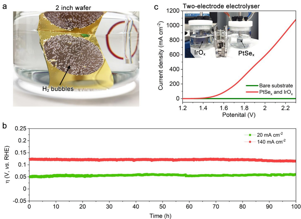
Figure 4. Wafer-scale fabrication and stability of amorphous PtSe_x catalyst. a , 2-inch amorphous PtSe_x film fabricated on an Au/SiO_2/Si substrate for mass production of hydrogen gas. b , Time-dependent overpotential ( \eta ) curves under j = 20\ mA\ cm^{-2} and 140\ mA\ cm^{-2} in 0.5\ M\ H_2SO_4 aqueous solution. c , Volt-ampere curves of overall water splitting in the two-electrode electrolyzer, made of an IrO_x anode and a PtSe_x cathode.
