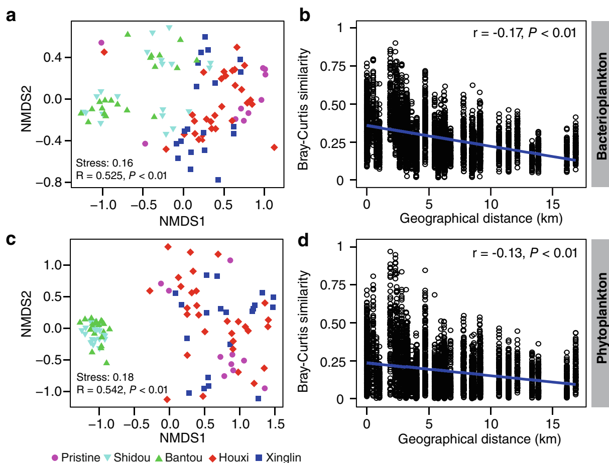
Fig. 3. Patterns of bacterioplankton and phytoplankton community similarity along the Houxi River, southeast China. Non-metric multidimensional scaling (NMDS) graphs visualizing (a) bacterioplankton and (c) phytoplankton communities based on Bray–Curtis similarity. The global R ( > 0.5 ) and its significant level ( p < 0.01 ) indicate the overall degree of sample separation across the five habitats along the river continuum over 5 yr. The distance–decay relationships of (b) bacterioplankton and (d) phytoplankton communities indicating the variation of community similarity along the geographical distance.
