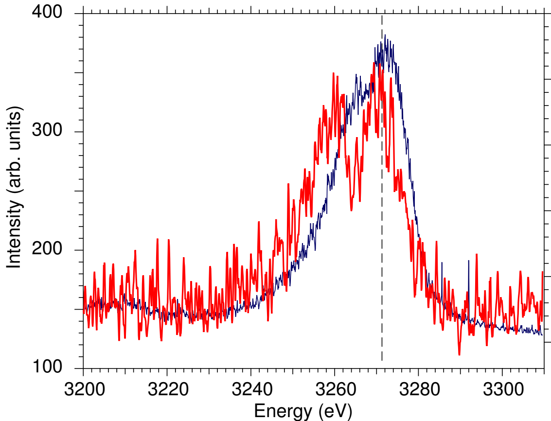
FIG. 3. Spectra showing the \text{Cl}^{15+} He- \beta line recorded with the OHREX spectrometer on the Orion laser and produced by short-pulse irradiation of a tamped PyD foil (blue trace, Orion shot 10140) and of a tamped KCl microdot (red trace, Orion shot 10142). The dashed vertical line indicates the location of the unshifted line. The vertical scale has been multiplied by 2 \times 10^4 relative to the scale shown in Fig. 2.
