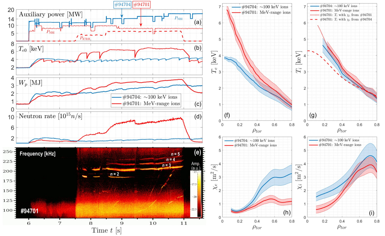
Figure 2: Demonstration of improved thermal ion confinement in fusion plasmas in the presence of MeV-range fast ions and destabilized TAEs. This is illustrated by comparing two JET pulses #94704 ( \sim 100 keV ions; blue lines) and #94701 (MeV-range ions; red lines) performed at the same operational conditions and the same total auxiliary heating power P_{\text{aux}} = 14 MW, but differing in the characteristics of the fast-ion population. (a) NBI and ICRF power. (b) Core electron temperature. (c) Plasma stored energy. (d) Neutron rate from D-D fusion reactions. (e) The magnetic coil spectrogram showing destabilized TAEs in pulse #94701. Panels (f) and (g) show the measured radial profiles of the electron, T_e and ion temperatures, T_i at P_{\text{aux}} = 14 MW. Panels (h) and (i) display the computed electron, \chi_e and thermal ion, \chi_i heat diffusivities. The red dotted and dashed lines in (g) show the two predicted T_i profiles in #94701, using \chi_i profiles from panel (i) as input. The error bars in (f) – (i) represent a combination of the systematic diagnostic uncertainties and time-averaged ( \pm 0.1 s) statistical variations of the measurements.
