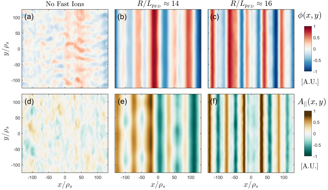
Figure 4: Evidence for the nonlinear generation of zonal structures. Contour plots of the gyroaveraged perturbed electrostatic potential, \phi and the component of the vector potential parallel to the magnetic field, A_{\parallel} . Panels (a) and (d) correspond to the case without fast ions; panels (b) and (e) - for the fast-ion case with R/L_{pFD} \approx 14 ; panels (c) and (f) - for the fast-ion case with R/L_{pFD} \approx 16 . All contour plots are normalized to the corresponding maximum value. This figure clearly shows the appearance of zonal structures leading to turbulence suppression in plasmas with MeV-range ions and fast-ion-driven TAEs.
