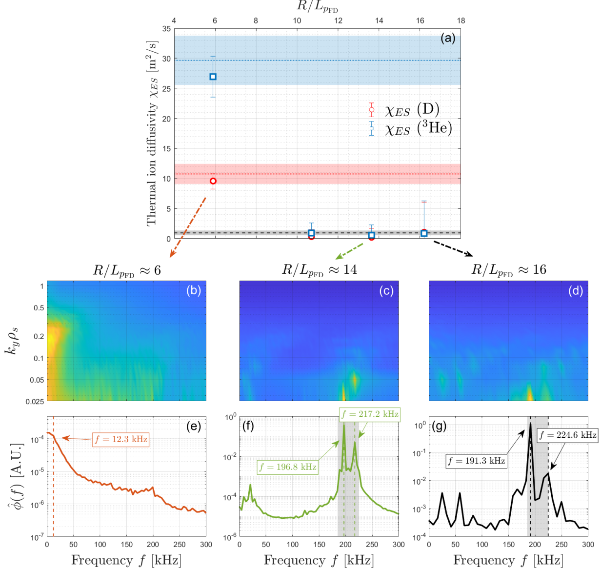
Figure 3: Illustration of thermal ion transport suppression in plasmas with MeV ions and fast-ion-driven modes. (a) The electrostatic thermal diffusivities of D and 3 He as predicted by GENE. (b-d) Amplitudes of the Fourier components of the perturbed electrostatic potential \hat{\phi} (averaged over the radial and parallel directions) as a function of frequency and k_y \rho_s . (e-g) The frequency dependence of \hat{\phi} , additionally averaged over k_y \rho_s . The error bars of GENE time-dependent simulations shown in panel (a) represent the standard deviation obtained from the code calculation. The large error bars for the rightmost points can be attributed to the high-frequency and large-amplitude modulations of the energy fluxes due to strong fast-ion-driven fluctuations of the electrostatic potential. In panel (a), thermal ion diffusivities and their standard deviations for the modelling case without fast ions are shown with the horizontal dotted lines and the associated shaded areas. The panel also shows the computed thermal ion heat diffusivity for JET pulse #94701, \chi_i = 0.8 \text{ m}^2 \text{ s}^{-1} as given by TRANSP (dashed line), with the grey shaded area representing the averaged uncertainty in the power balance computation by TRANSP (see also the Methods section).
