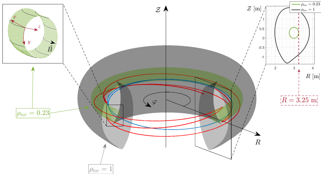
Figure 1: Schematic view of the tokamak geometry. In tokamaks, charged particles are confined by a combination of toroidal and poloidal magnetic fields that generate nested magnetic surfaces of constant magnetic flux needed for plasma confinement. Passing particles (blue trajectory) circulate along magnetic field lines in the toroidal direction \varphi , while trapped particles (red trajectory) periodically reverse their parallel velocity. For simplicity, the rapid gyromotion of charged particles is omitted and only the guiding center motion is shown. In this paper, the local transport analysis focuses at the magnetic flux surface corresponding to \rho_{\text{tor}} = 0.23 (in green), where \rho_{\text{tor}} is the square root of the toroidal magnetic flux normalized to its value at the plasma boundary. The inset at the top on the left illustrates the field-aligned set of coordinates used in the flux-tube version of the GENE code, with (x, y, z) the radial, binormal and parallel coordinate, respectively. The figure at the top on the right shows a poloidal cross-section of the plasma in the (R, Z) plane, where R is the radial distance from the torus centre and Z is the vertical coordinate; the flux surface for \rho_{\text{tor}} = 0.23 (green) and \rho_{\text{tor}} = 1 (black) are also illustrated.
