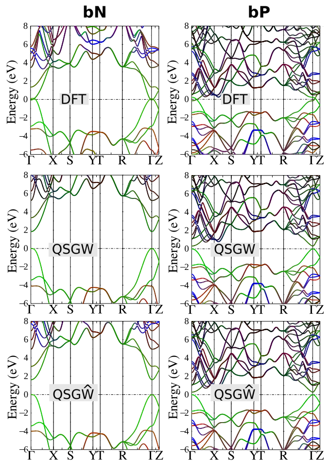
FIG. 3. Single-particle band structure of BN (left) and BP (right) calculated using the DFT (LDA), QSGW, and QSGW ̂ approaches (from top to bottom) along high-symmetry directions of the conventional Brillouin zone (Fig. 1). The colors correspond to the contributions of p_x (blue), p_y (red), and p_z (green) orbitals.
