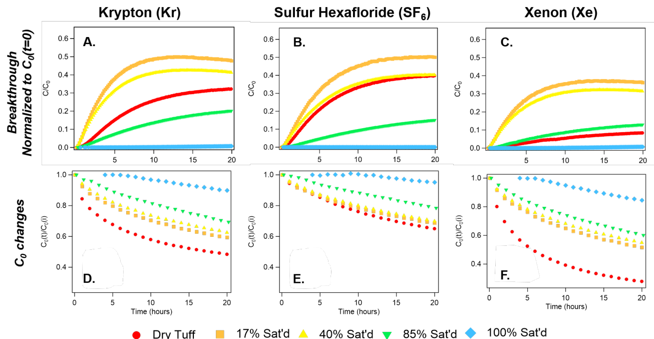
Figure 3. Diffusion breakthrough curves for (A) Kr, (B) SF 6 , and (C) Xe, normalized to the initial measured C 0 (C 0 (t=0)); Changes in the spiked concentration with time for (D) Kr, (E) SF 6 , and (F) Xe.
