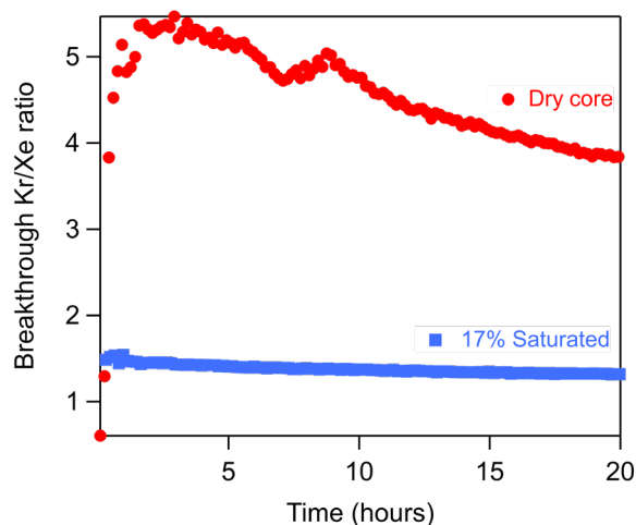
Figure 7. Ratio of Kr/Xe breaking through core over the 20 hour diffusion study. A much higher ratio is present in the dry core due to low Xe diffusion and more significant Xe sorption.
