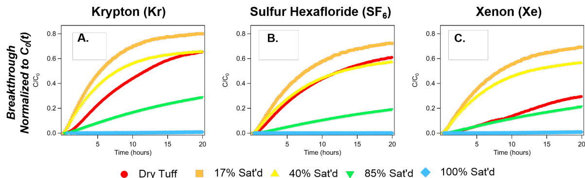
Figure 5. Diffusion breakthrough curves for (A) Kr, (B) SF 6 , and (C) Xe, normalized to the measured C_0 at each time point, C_0(t) .
