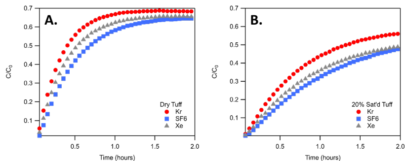
Figure 4. Diffusion of Kr, SF 6 , and Xe were measured through a tuff core which did not contain zeolites under (A) dry and (B) 20% saturated conditions.
