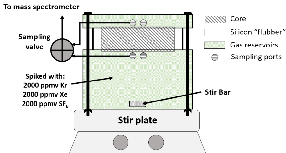
Figure 2. Diffusion cell schematic
