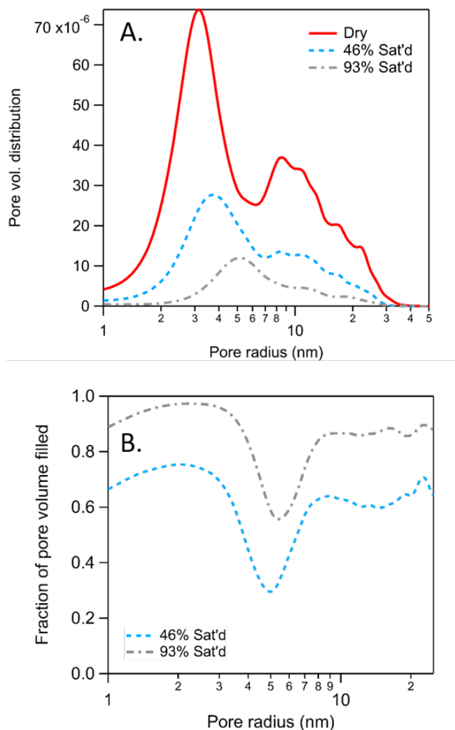
Figure 6. (A) Fitted pore size distribution for zeolitic tuff with increasing water content, showing that smaller pores will preferentially fill first. Fitting used Irena's maximum entropy method. Comparison between fitting methods can be found in the SI. (B) Fraction of filled pores across the fitted size range. Size is cut off at 25 nm because ratios become skewed as the distribution approaches zero.
