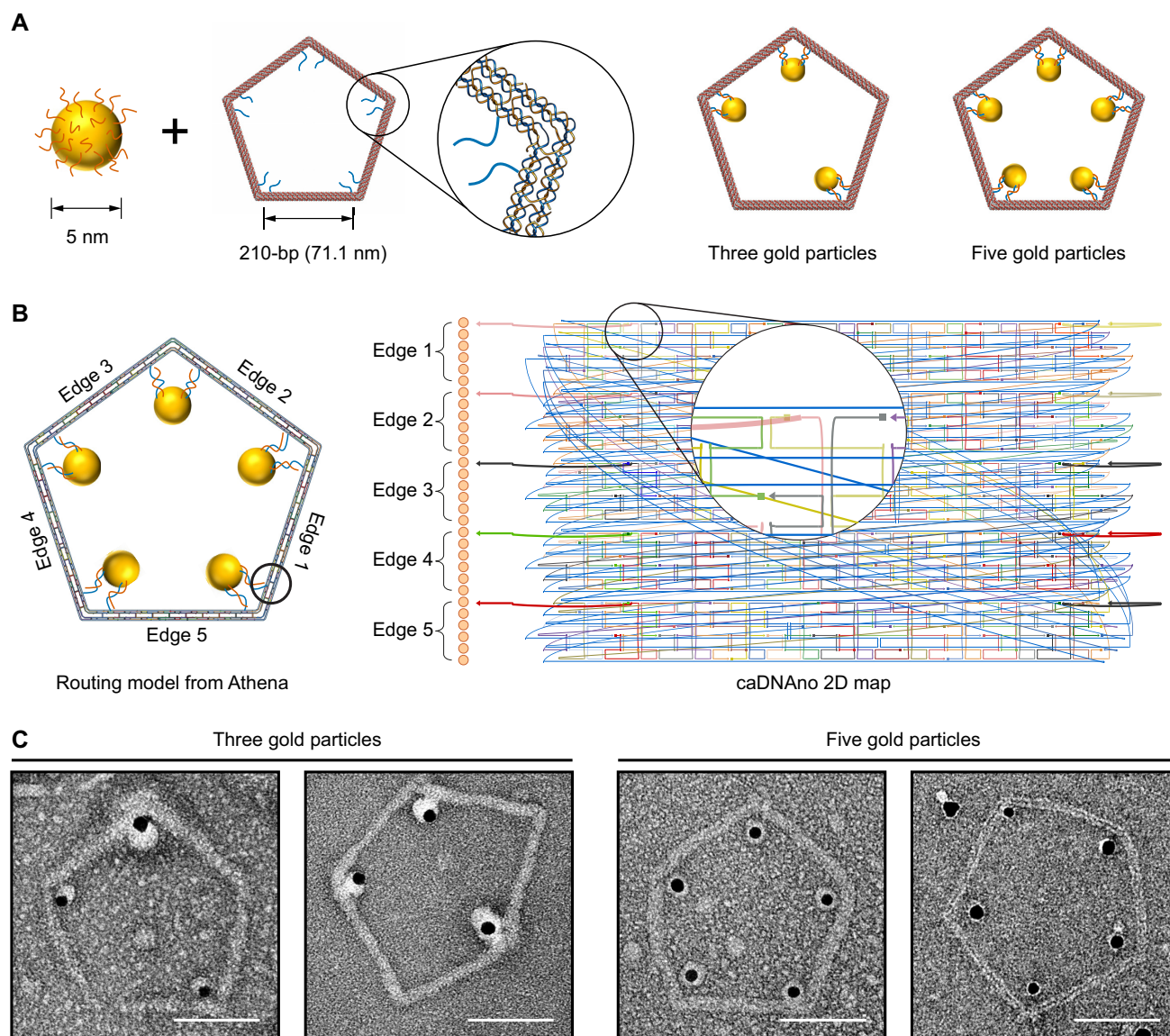
Figure 5. Organizing AuNPs on the 210-bp pentagonal DNA origami. (A) Diagrams showing the attachment of NPs at three or five corners. (B) Routing model and caDNAAno representation for pentagonal DNA origami with AuNPs. (C) TEM images with 2D pentagonal DNA origami of organized AuNPs. Scale bars, 50 nm.
