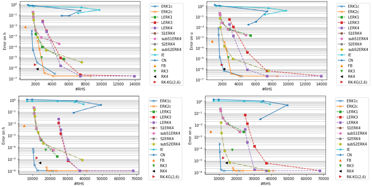
Figure 15: Space time source term test case. Same as Figure 12. C4 spatial discretization.
