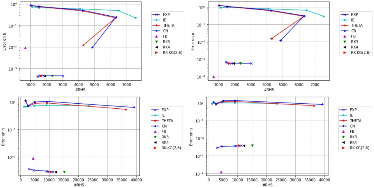
Figure 8: Linear test case. Relative error as a function of the number of right hand side (RHS) evaluations (which is itself given by the choice of the time step). The period of integration is T = 6 hours. On the top panels, we consider the shallow ocean \bar{h} = 100 meters; on the bottom panels, the deep ocean with \bar{h} = 4000 meters. The spatial discretization scheme is C2.
