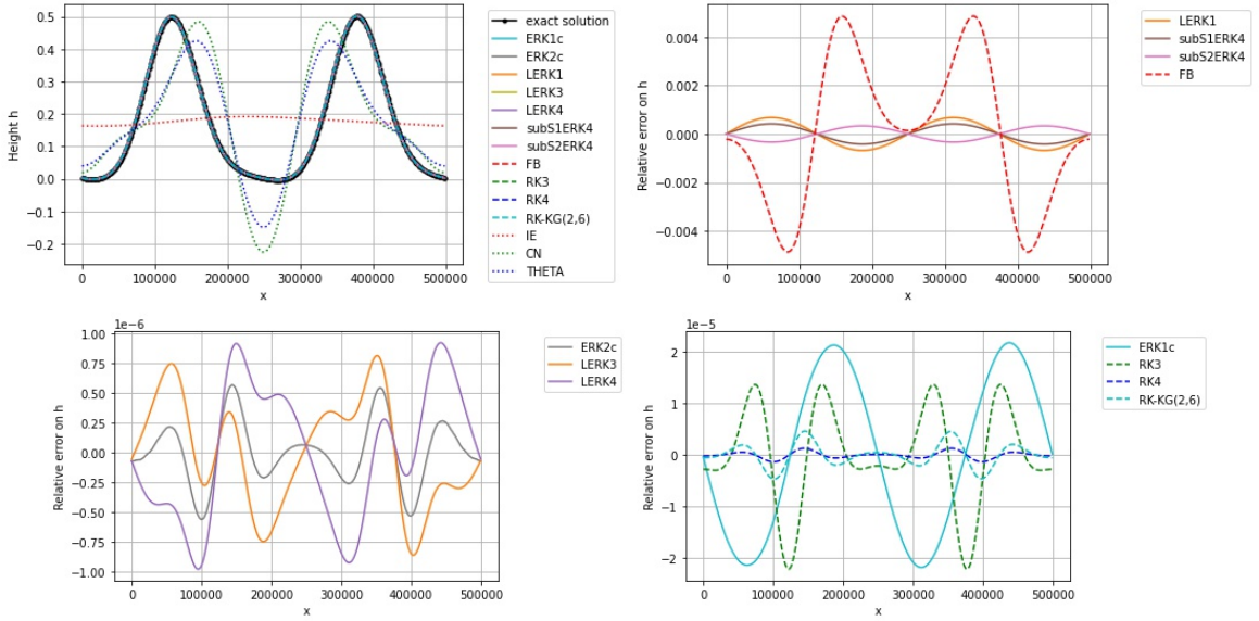
Figure 13: Spatio-temporal source term test case. Numerical solution h computed using fourth order C4 spatial discretization with \bar{h} = 100\text{m} (shallow ocean). First plot (top left): solution h at t = 10 hours. Three next plots: relative errors on h . A-stable schemes have \Delta t = 600\text{s} , Explicit schemes time steps \Delta t_{\text{RK4}} = 30\text{s} , \Delta t_{\text{FB}} = \Delta t_{\text{RK3}} = 20\text{s} and \Delta t_{\text{RK-KG}(2,6)} = 60\text{s} .
