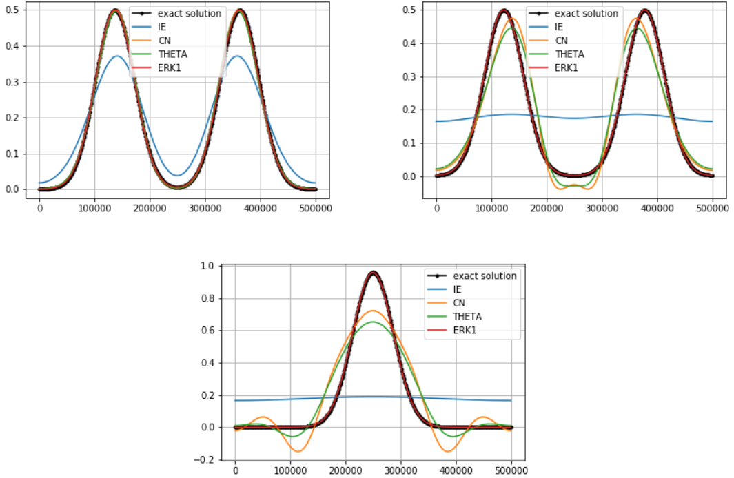
Figure 7: Linear test case. Numerical solutions \eta computed using C4 spatial operators and \bar{h} = 100 meters. \Delta t = 300s ( c\Delta t/\Delta x = 9.4 ). Top left panel: solution at t = 1h . Top right panel: solution at t = 10h . Bottom panel: solution at t = 40h .
