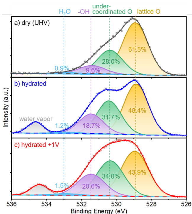
Figure 2. O 1s spectra for BZY at three conditions, deconvoluted by four peaks with same width and constrained position: lattice O (yellow, 528.9 eV); undercoordinated O (green, 530.4 eV); hydroxyl group -OH (violet, 531.4 eV); adsorbed intact H 2 O (blue, 533.0 eV).
