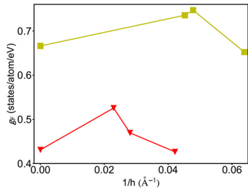
Figure 8. Number of states at the Fermi level as a function of the inverse of the thickness in \alpha -Nb 5 Si 3 (red) and Nb 6 Si 5 (yellow). Here, the states are counted only from Nb in the structure we computed at each thickness for an accurate prediction of the changes of metallicity, because almost all of the DOS at the Fermi level is from Nb.
