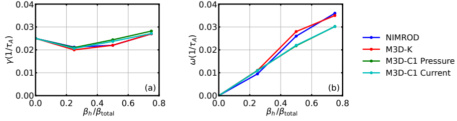
Figure 3: Simulation results of mode growth rate (a) and real frequency (b) as functions of EP beta fraction of the n = 1 fishbone. Blue line is the result of NIMROD[3]. Red line is the result of M3D-K[2]. Green line is the result of M3D-C1-K using pressure coupling, and the cyan line is the result using current coupling.
