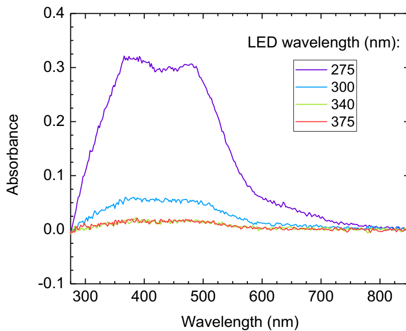
Figure 4. Absorbance spectra of \beta -Ga 2 O 3 :Cu samples that were exposed to LEDs of different wavelengths. Significant photodarkening is observed for the 300 and 275 nm LEDs. Sample thicknesses were 0.67 mm (same sample for 375 and 275 nm exposures), 0.49 mm (340 nm exposure, same sample as Fig. 2), and 0.45 mm (300 nm exposure).
