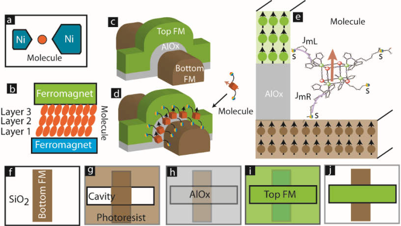
Figure 1: Conceptual representation of conventional (a) nanogap breakjunction, and (b) sandwiched type MSD. MTJMSD 3D-architecture (c) before and (d) after magnetic molecules treatment (e) 3D MTJMSD model analogues to MTJMSD in panel (d). MTJMSD fabrication flow is based on (f) depositing bottom electrode in photolithographically defined cavity, (g) photolithography for (h) AlOx insulator, (i) top electrode. (j) Liftoff producing exposed edge MTJ
