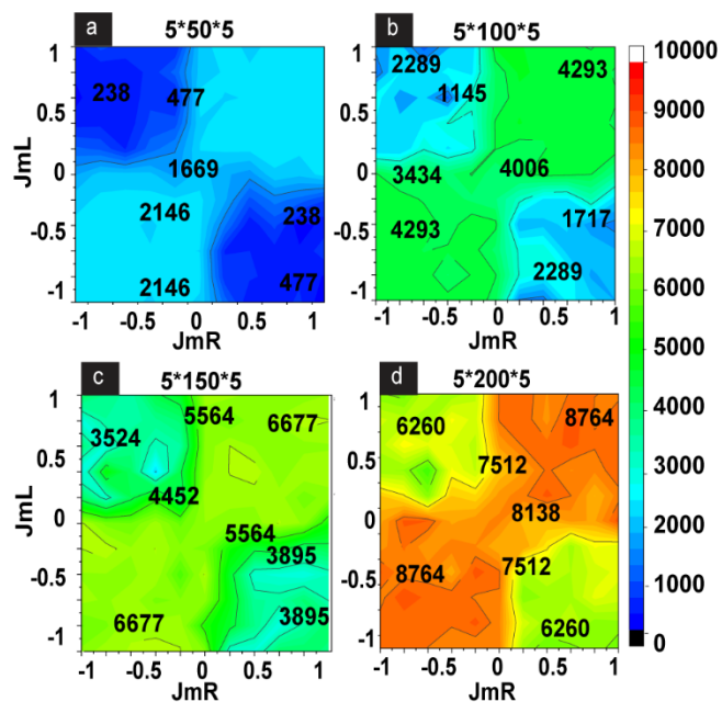
Figure 7: Total MTJMSD's Magnetic Moment for increased length devices (a) 5*50*5, (b) 5*100*5 (c) 5*150*5 (d) 5*200*5
