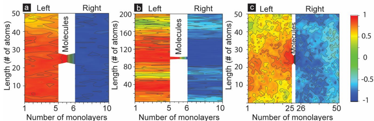
Figure 6: Correlation factor contour plots of MTJMSD for all layers of left and right FM electrodes and the magnetic molecule when J_{mL} = 1 , J_{mR} = -1 , for device with FM electrodes of (a) 50 atom length and 5 atom thickness, (b) 200 atom length and 5 atom thickness (c) 50 atom length and 25 atom thickness. Width of FM electrode was 5 atom.
