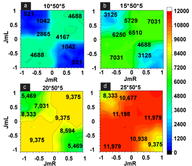
Figure 8: Total MTJMSD's Magnetic Moment for increased widths devices (a) 10*50*5 , (b) 15*50*5 (c) 20*50*5 (d) 25*50*5
