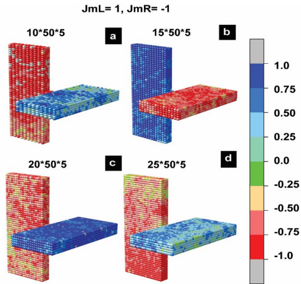
Figure 5: 3D Lattice plot of MTJMSD' s Magnetic Moment when JmL=1 and JmR= -1 for increased thickness devices (a) 10*50*5 , (b) 15*50*5 (c) 20*50*5 (d) 25*50*5
