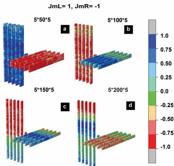
Figure 4: 3D Lattice plot of MTJMSD' s Magnetic Moment when JmL=1 and JmR= -1 for increased length devices (a) 5*50*5 , (b) 5*100*5 (c) 5*150*5 (d) 5*200*5
