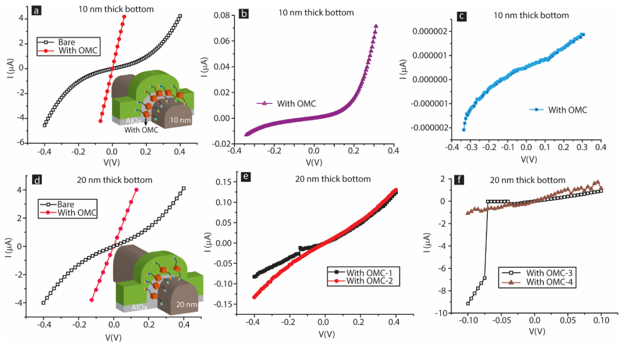
Figure 2: MTJMSD with 10 nm bottom electrode showing (a) tunneling transport on bare MTJ and the highest current value observed, (b) asymmetric nA range suppressed state, (c) pA level suppressed current state. MTJMSD with \sim 20 nm thick bottom FM electrode showing (d) tunneling transport on bare MTJ and the highest current value observed, (e) nA range suppressed state, and (f) instability leading to high and low current state.
