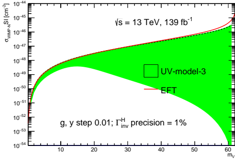
FIGURE 4: Green bands of upper limit on \sigma^{\text{SI}}(\text{V-N}) from coarse scan in Table 2 (upper canvas), fine scan from Table 3 (middle), and fine scan from Table 3 with looser precision of \Gamma_{\text{inv}}^{\text{H}} (down canvas) are shown in comparison with EFT red line, for the UV model in [27].
