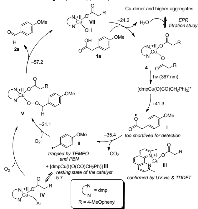
Scheme 2. Proposed Mechanism based on experimental and computational investigations. \Delta_rG values of each indicated step in kcal/mol.
