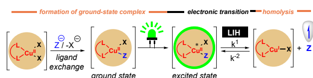
Figure 1. Concept of light induced homolysis (LIH) for Cu(II)-species)
