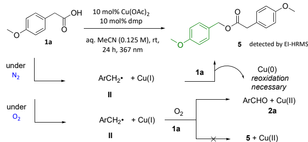
Scheme 3. Cu(II)-mediated decarboxylation under oxygen and inert gas atmosphere.
