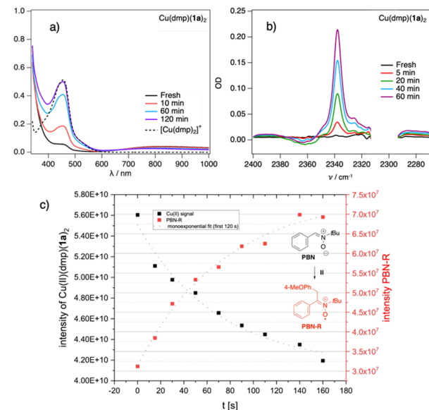
Figure 3. a) UV-Vis absorption spectra of fresh and irradiated Cu(dmp)( 1a ) 2 ( 3 ), and independently prepared [Cu(dmp) 2 ] + (dashed line) as reference; b) Solution-phase IR spectra of fresh and irradiated Cu(dmp)( 1a ) 2 ( 3 ) showing the emergence of the CO 2 absorbance band at 2335 cm -1 growing with irradiation time; c) Kinetic traces of Cu(II) signal (black squares) with k_{\text{initial}} = 0.015 \pm 0.004 s -1 and of the growth of the PBN-R signals (red squares) with k_{\text{initial}} = 0.013 \pm 0.002 s -1 . Fitted at early times with a single exponential
