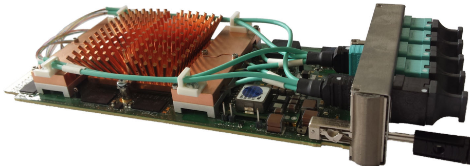
Figure 21: LATOME board equipped with optical fibers.
