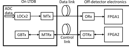
Figure 8: Block diagram of the LTDB optical links.
