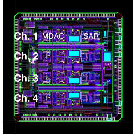
Figure 7: Image of ADC layout ( 3.6 \times 3.6 mm).
