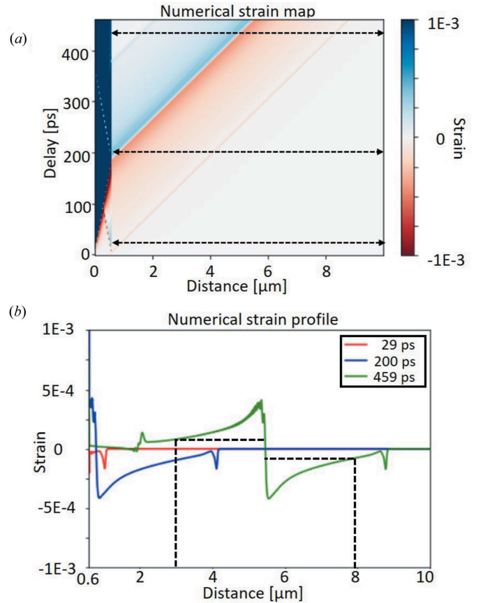
Figure 2 Strain-wave profile in a diamond single crystal as a function of time delay from laser pulse heating, as computed using a 1D thermomechanical model. (a) 2D map of strain versus depth and time delay. (b) 1D plots of the strain profile in diamond at different time delays [indicated with dashed lines in (a)]. The spatial extent of the part of the strain wave that is visible in DFXM at 459 ps (indicated with dashed lines) is about 5 \mu\text{m} .
