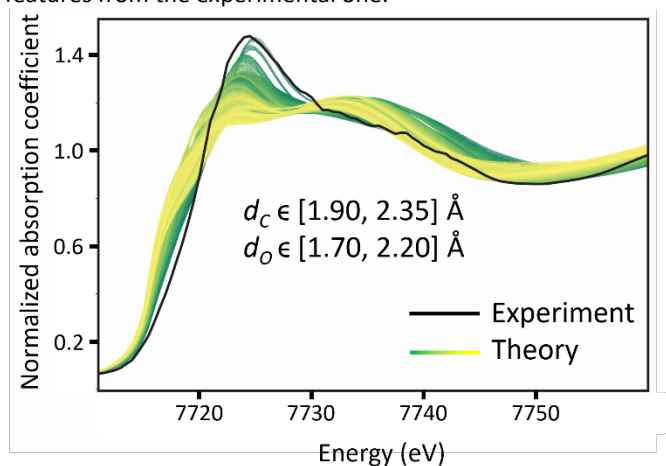
Figure 8. Comparison between the experimental XANES spectrum of Co-cyclam-CO (black) and all the theoretical XANES spectra. The spectra with the colour from green to yellow are simulated XANES with two descriptors changing ( d_C and d_O ).
