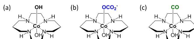
Figure 6. Proposed structures of Co(III) complex related to CO 2 reduction on Co-cyclam/C 3 N 4 , including the fresh sample(a), the sample with TEOA and CO 2 before light (b), the sample at the end of the reaction (the product structure, c).
