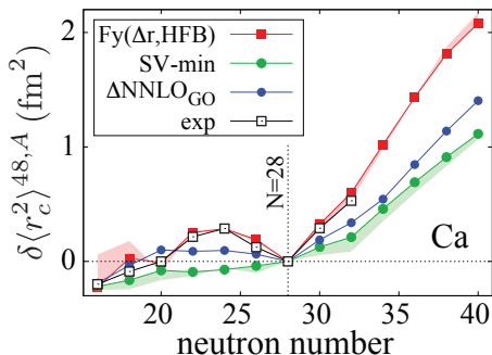
Figure 4. Differential radii of the Ca isotopes. Theoretical uncertainties for CC calculations are discussed in the text.
