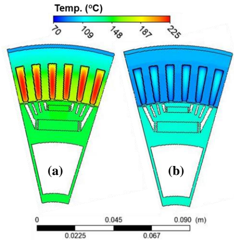
Figure 14: Temperature contour of (a) JC and (b) EC at rms current density of 18 A/mm 2 , constant shaft speed of 4500 rpm, and phase advance of 45 EDeg. In case of JC, coolant flow rate was 10 L/min (corresponding h was 5,054 W/m 2 .K), whereas in case of EC, h_{eva} was 5,000 W/m 2 .K.
