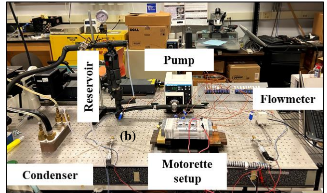
Figure 25: (a) Schematic of the flow loop (b) actual setup with the motorette in the two phase loop.
