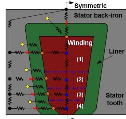
Figure 7: Schematic of resistance network of single slot, liner, and the corresponding stator lamination for EC (schematic not drawn to scale). Red resistance indicate liner-lamination contact resistance and yellow nodes are set at constant saturation temperature of 80^\circ\text{C} .
