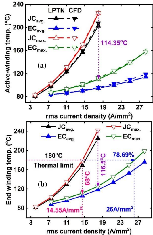
Figure 12: Steady-state (a) active-winding and (b) end-winding temperature vs. rms current density for JC and EC at constant shaft speed of 4500 \text{ rpm} and phase advance of 45 \text{ EDeg} . In case of JC, coolant flow rate was 10 \text{ L/min} (corresponding h was 5,054 \text{ W/m}^2\text{K} ), whereas in case of EC, h_{eva} was 5,000 \text{ W/m}^2\text{K} . Lowest current density of 4.10 \text{ A/mm}^2 has not been considered for EC and the end-winding temperature has been calculated from the LPTN model only.
