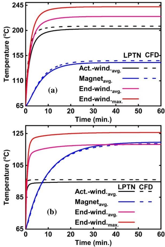
Figure 18: Temporal evolution of temperature for (a) JC, and (b) EC at constant current density of 18 A/mm 2 (which corresponds to peak operating condition for JC), initial temperature of 65°C, shaft speed of 4500 rpm, and phase advance of 45 EDeg. In case of JC, coolant flow rate was 10 L/min (corresponding h was 5,054 W/m 2 .K), whereas in case of EC, h_{eva} was 5,000 W/m 2 .K.
