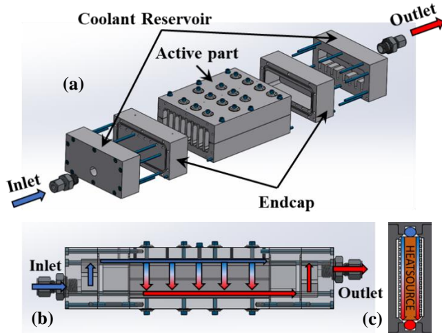
Figure 24: (a) Expanded view of the motorette assembly, (b) schematic of coolant flow path through the testbed, and (c) front view of a single slot.
