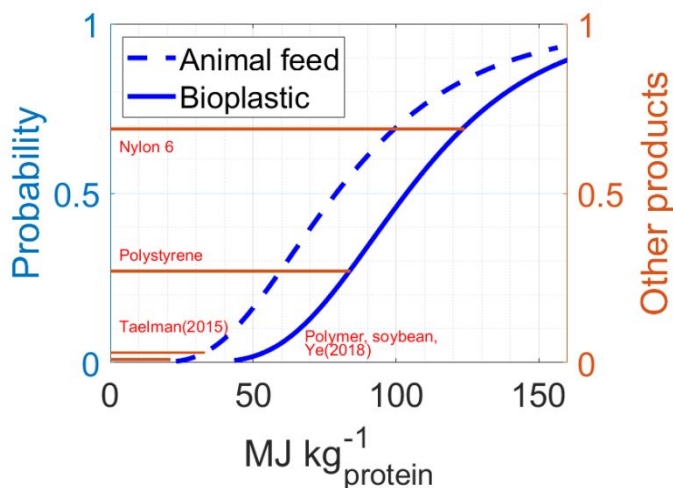
Figure 3. Lognormal probabilistic distribution of high-protein algal-derived animal feed (dashed-line) and polymer (continuous-line) life cycle energy. Algae-derived animal feed life-cycle energy probabilistic distribution was compared against metrics reported in the literature, including algae-derived animal feed and soybean 59, 79, 298 . Algae-derived bioplastics life-cycle energy probabilistic distribution was compared against products reported in the literature, including nylon 6, polystyrene, and polymer 298 .
