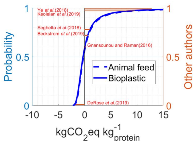
Figure 4. Stable probabilistic distribution of high-protein algal-derived animal feed (dashed-line) and polymer (continuous-line) life cycle CO 2 eq emissions. Life cycle CO 2 eq probabilistic distribution is compared against metrics reported in the literature including algal-derived animal feed 20, 58, 59, 80, 298 and algae-derived bioplastic 56 .
