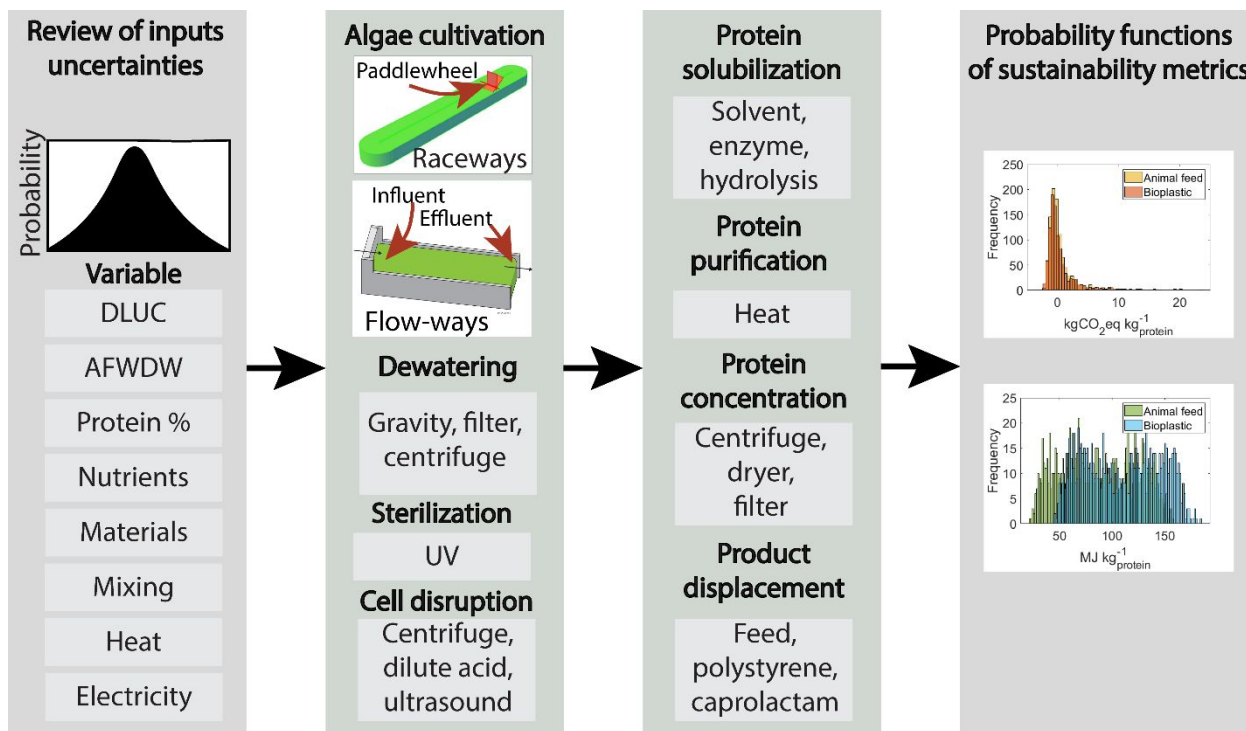
Figure 1. High-protein algae bioproducts system boundaries for environmental sustainability risk analysis. The first algae-derived animal feed system considers model input uncertainties for algae cultivation, biomass dewatering, biomass sterilization, cell disruption, protein purification, and concentration. The second algae-derived polymer system considers additional product preparation unit processes, including membrane separation, microwave processing, and jet milling. DLUC: Direct-land Used Change. AFWDW: Ash-free dry weight biomass.
