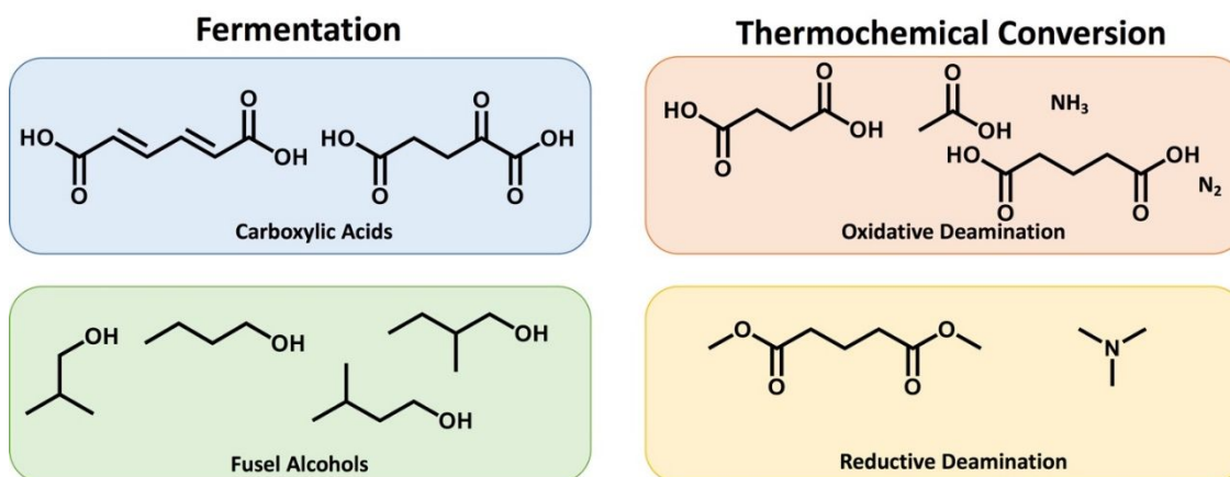
Figure 2. Overview of molecular structure of biochemical and thermochemical protein-derived small molecule conversion products as described in the text.
