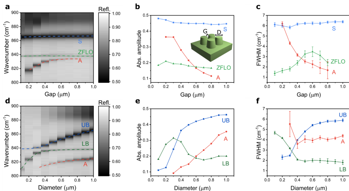
Figure 2: Tuning of the symmetric and antisymmetric modes in 2x2 subarray. Experimental dispersion plot made of reflection spectra for 2x2 structure with different gaps in the unit cell (a) and different nanopillar diameters (d). Peak positions from Lorentz fitting of the experimental spectra are plotted on top of the dispersion plots in (a) and (d) to better illustrate. Absorption amplitude of the investigated modes for 2x2 structure with different gaps in the unit cell (b) and different pillar diameters (e). Linewidth (FWHM) of the investigated modes for 2x2 structure with different gaps in the unit cell (c) and different pillar diameters (f). Inset in (b) illustrates the tuning parameters (gap: G and diameter: D). The error bars in (c) and (f) are the uncertainty from the Lorentz fitting of the reflection dips. For the 2x2 structure with different gaps, the period of the unit cell is 6 \mu\text{m} and the pillar diameter is 1 \mu\text{m} . For the 2x2 structure with different diameters, the period of the unit cell is 6 \mu\text{m} and the gap in the unit cell is 0.3 \mu\text{m} .
