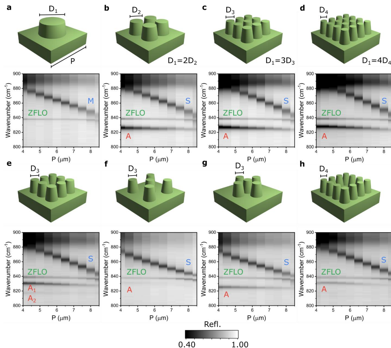
Figure 3: The experimental dispersions of symmetric and antisymmetric modes in the complex subarrays. Experimental dispersion plots made of reflection spectra with different unit cell periods for (a) 1x1 structure, (b) 2x2 structure, (c) square 3x3 structure, (d) square 4x4 structure, (e) 3x3 structure without the center pillar, (f) 3x3 structure features as X-shape, (g) 3x3 structure features as cross-shape, (h) 4x4 structure without center 2x2 pillars.
