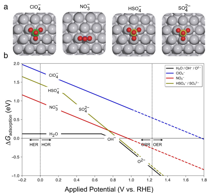
Figure 3: Potential dependent anion adsorption on Pt(111) surface. (a) The most stable adsorption configurations of anions on the Pt(111) surface. Color coded: O: red, H: white, Cl: green, N: blue, and S: yellow. (b) The adsorption free energies of the anions, \Delta G_{\text{adsorption}}(A^{n-}) (eV), on the Pt(111) surface as a function of applied potential (V vs. RHE). The colored dashed lines qualitatively shows the trends in \Delta G_{\text{adsorption}}(A^{n-}) at higher potentials relevant for the oxygen evolution reaction (OER). Since the Pt(111) surface undergoes surface oxidation at these high potentials, we further calculated \Delta G_{\text{adsorption}}(A^{n-}) trends on a \text{PtO}_2(110) surface as shown in Supplementary Figure 5 and Table 4 . Anion species color-coded: black ( \text{H}_2\text{O}/\text{OH}^-/\text{O}^{2-} ), blue ( \text{ClO}_4^- ), red ( \text{NO}_3^- ), and yellow ( \text{HSO}_4^-/\text{SO}_4^{2-} ). HER/HOR, and ORR/OER stand for hydrogen evolution/oxidation reaction and oxygen reduction reaction, respectively.
