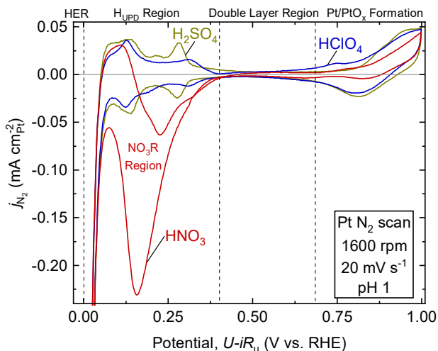
Figure 1: Characteristic Pt cyclic voltammogram in N 2 -saturated HClO 4 , H 2 SO 4 , and HNO 3 . Representative cyclic voltammogram (CV) of Pt disk at 20 mV sec -1 in N 2 -sat'ed HClO 4 , H 2 SO 4 , and HNO 3 . Dashed regions indicate approximate divisions of potential ranges indicated along the top: hydrogen evolution reaction (HER) region, hydrogen under-potential deposition (H UPD ) region, double layer capacitance region, and surface Pt oxidation/PtO x reduction region. Color code: HClO 4 (blue), HNO 3 (red), and H 2 SO 4 (yellow).
