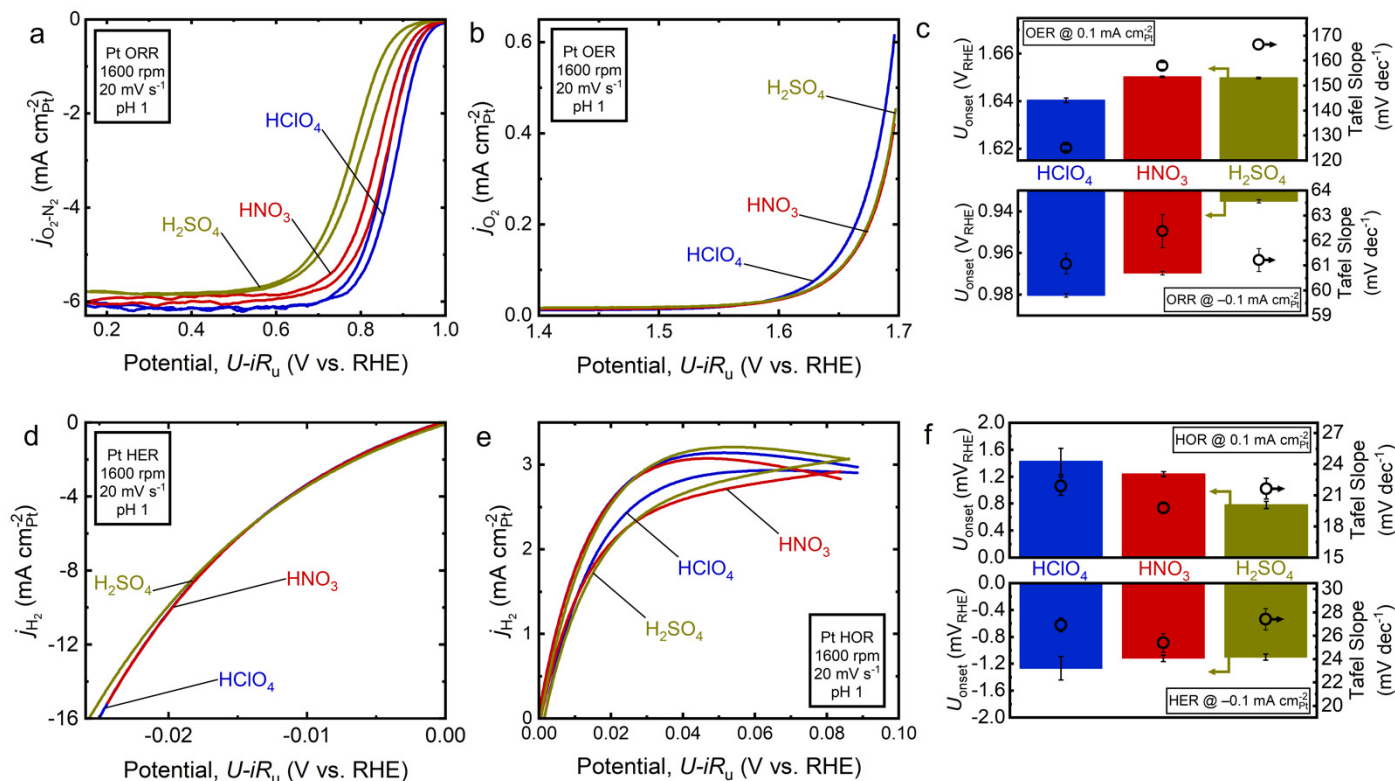
Figure 2: Evaluation of Pt for oxygen and hydrogen electrocatalysis in HClO 4 , HNO 3 , and H 2 SO 4 . (a) Representative third-cycle-averaged N 2 -subtracted oxygen reduction reaction (ORR) rotating disk electrode (RDE) cyclic voltammogram (CV) of the Pt disk in pH 1 HClO 4 , HNO 3 , and H 2 SO 4 . (b) Representative second-cycle-averaged oxygen evolution reaction (OER) RDE CV of the Pt disk in pH 1 HClO 4 , HNO 3 , and H 2 SO 4 (OER trend is consistent as a function of cycle, Supplementary Fig. 4 ). (c) Average OER (top) and ORR (bottom) onset potential (bars, left y-axis) \pm 0.1 mA cm -2 for all three acids and average Tafel slope (circles, right y-axis) in the low current density region. (d) Representative third-cycle-averaged hydrogen evolution reaction (HER) RDE CV of the Pt disk in pH 1 HClO 4 , HNO 3 , and H 2 SO 4 collected. (e) Representative third-cycle-averaged hydrogen oxidation reaction (HOR) RDE CV of Pt disk in pH 1 HClO 4 , HNO 3 , and H 2 SO 4 . (f) Average HOR (top) and HER (bottom) onset potential (bars, left y-axis) \pm 0.1 mA cm -2 for all three acids and average Tafel slope (circles, right y-axis) in the low current density region. Error bars represent the standard deviation of separate triplicate measurements. All CVs collected at 1600 rpm, 20 mV sec -1 , and iR_u corrected. Color code: HClO 4 (blue), HNO 3 (red), and H 2 SO 4 (yellow).
