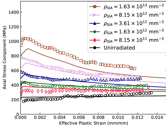
Fig. 6: Comparison of crystal plasticity simulations with dislocation dynamics simulations of the stress-plastic strain evolution, with the varying initial values for SIA loop densities demonstrating trends similar to those in [37] particularly at the lower initial SIA loop densities. Here we focus on the alignment of the trends given the underlying differences in the discrete dislocation dynamics and continuum-level crystal plasticity frameworks, limited by the strain values from dislocation dynamics simulations. The dislocation dynamics data (represented with hollow markers) are reproduced from [16]; our crystal plasticity simulation results are represented by the solid lines.
