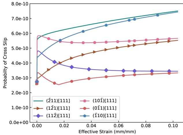
(a) Probability of cross slip in the [111] cross slip family
