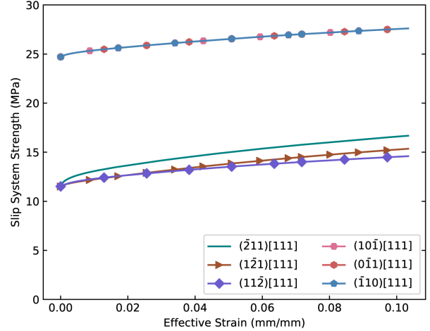
(b) Slip system strength evolution in the [111] cross slip family
