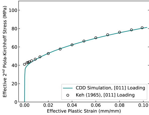
(b) Comparison of the CDD model in the [0\bar{1}\bar{1}] loading direction using the \alpha values given in Tab. 2 with single-crystal BCC \alpha -iron
