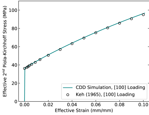
(a) Verification in the [100] loading direction of the dislocation-mechanism term \alpha coefficients against single-crystal BCC \alpha -iron
