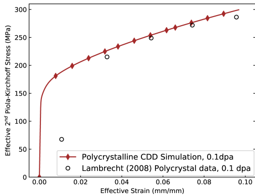
(b) CDD model predictions for radiated (0.1 dpa) polycrystalline \alpha -iron
