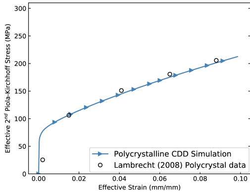
(a) CDD model predictions for unirradiated polycrystalline \alpha -iron
