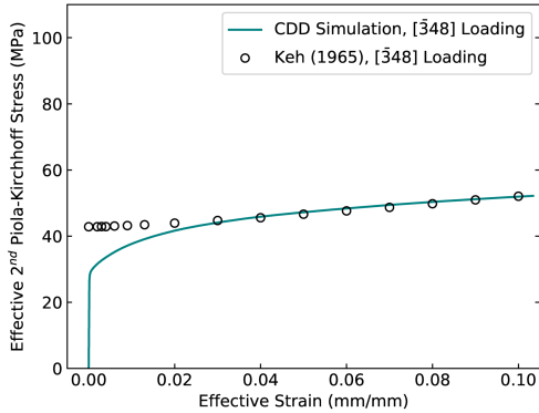
(c) Demonstration in the [\bar{3}48] loading direction of the dislocation evolution mechanisms \alpha coefficients against single-crystal BCC \alpha -iron
