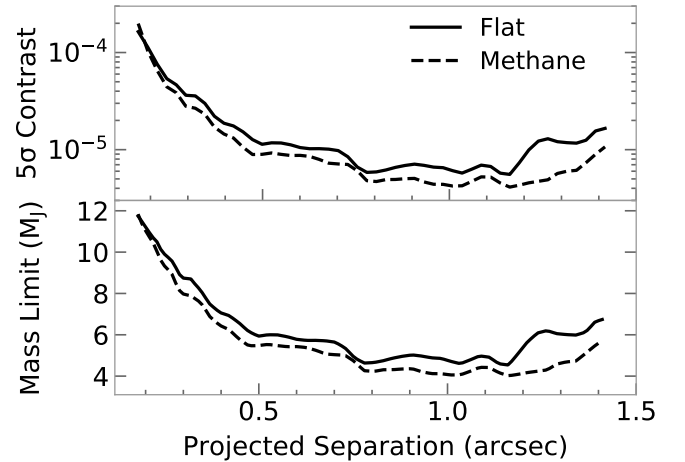
Figure 5. Top: The 5\sigma contrast limits from our H-Spec data, assuming either a flat or methane-absorption planet spectrum. Bottom: The contrasts are converted to mass limits for “hot start” planets.
