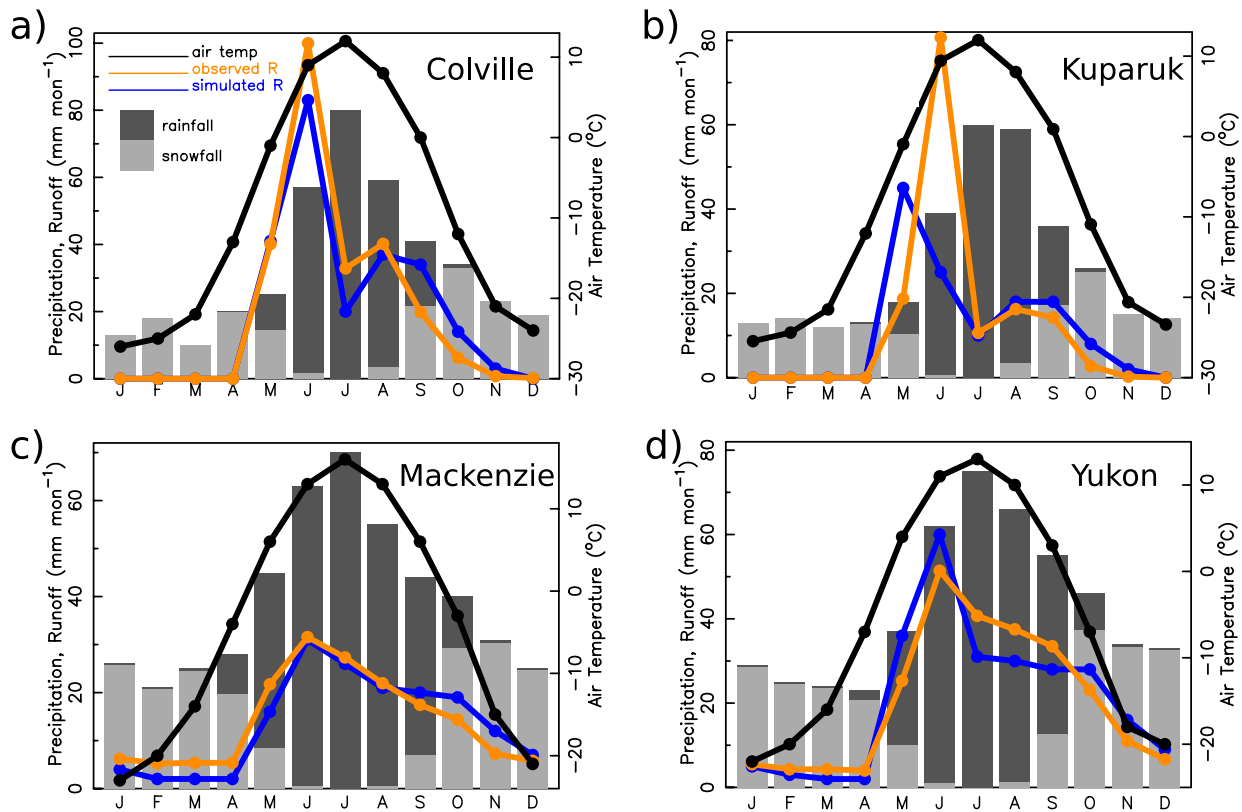
Figure 3. Monthly precipitation ( \text{mm mon}^{-1} ), runoff ( \text{mm mon}^{-1} ), and air temperature ( ^{\circ}\text{C} ) as climatological averages over the period 1981–2010 from the baseline simulation for the (a) Colville, (b) Kuparuk, (c) Mackenzie, and (d) Yukon River basins. Runoff is expressed in unit depth equivalent. Observed runoff in unit depth was obtained by distributing the measured river discharge flux volumes across the contributing basin area.
