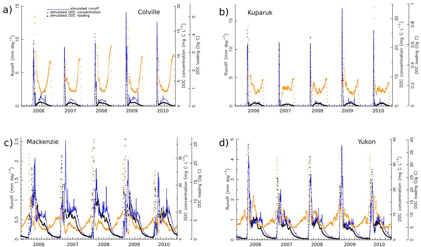
Figure 5. Daily simulated runoff ( \text{mm day}^{-1} ), DOC concentration of leachate ( \text{mg C L}^{-1} ), and DOC loading ( \text{Gg C} ) for the four focus basins during 2006–2010.
