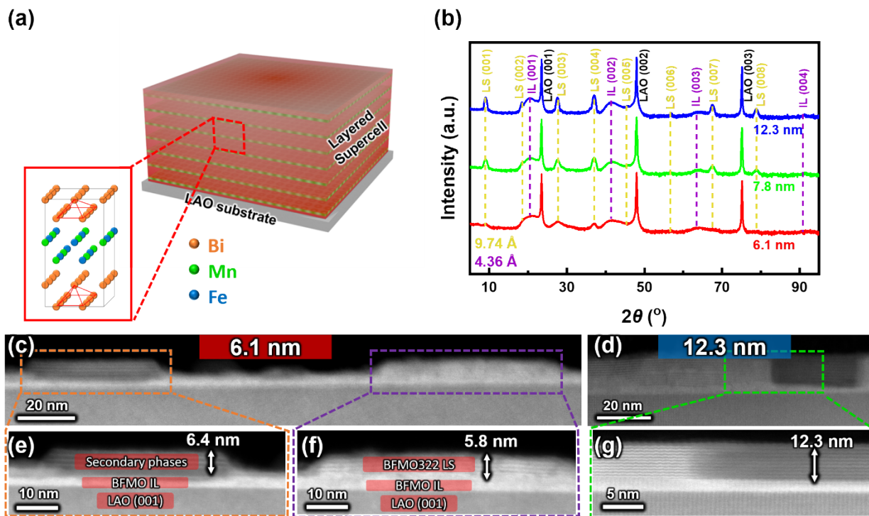
Figure 1. Microstructural characterization. (a) Schematic diagram of the Bi 3 Fe 2 Mn 2 O 10+δ layered supercell (BFMO322 LS) structure. The enlarged schematic illustrates atomic modeling of the BFMO322 cation sublattice. (b) XRD \theta - 2\theta scans of BFMO films at three thicknesses showing two sets of (00l) peaks with different lattice constants, corresponding to the BFMO322 LS (yellow dashed line) and the BFMO interlayer (IL) with pseudo-perovskite structure (purple dashed line), respectively. (c, d) Cross-sectional low-magnification STEM HAADF images of the 6.1 nm and 12.3 nm BFMO films, respectively. (e, f, g) STEM HAADF images of the marked region in (c, d), illustrating the morphology of films with different thicknesses.
