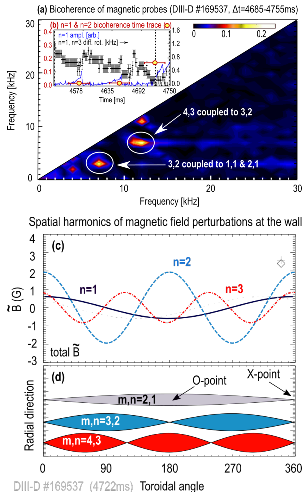
FIG. 2: (a) Bi-coherence of \tilde{B}_\theta at the time of 2,1 seeding. (b) Time trace of bicoherence between the n = 1 & n = 2 modes, n = 1 amplitude and differential rotation of n = 1 and n = 3 modes. (c) Spatial harmonics of \tilde{B}_\theta . (d) Cartoon of 2,1, 3,2 and 4,3 islands with phasing derived from (c).
