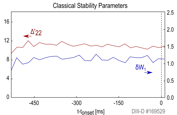
FIG. 3: \delta W_1 & \Delta'_{22} . Positive values reflect stable conditions.
