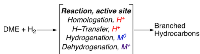
Fig. 1. Schematic of reaction pathways and corresponding active sites for DME homologation with co-fed \text{H}_2 over metal-modified BEA zeolite catalysts.
