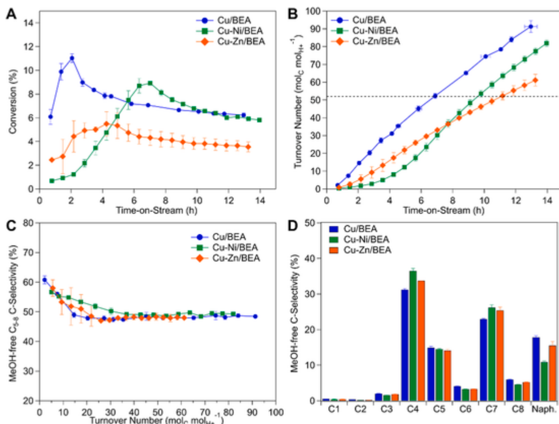
Fig. 5. Plots from DME homologation over Cu/BEA, Cu-Zn/BEA and Cu-Ni/BEA for (A) conversion and (B) TON versus TOS with TON = 52 indicated with a horizontal dashed line. Methanol-free carbon-selectivity for (C) total high-octane gasoline range C 5-8 hydrocarbons versus TON, and (D) hydrocarbon distribution by carbon number taken at TON = 52 ± 2 mol C mol H + -1 . Reaction conditions were 200 °C, 103 kPa, DME WHSV of 2.2 h -1 , p DME and p H 2 each 47 kPa, remainder p Ar . Data are presented as mean ± SEM for Cu/BEA and mean ± range for Cu-Ni/BEA and Cu-Zn/BEA.
