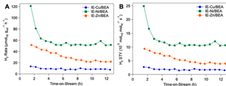
Fig. 2. (A) H_2 formation rate and (B) STY of H_2 over IE-M/BEA catalysts during isobutane dehydrogenation as a function of TOS. Reaction performed at 300 °C, 200 kPa, isobutane WHSV of 0.10 \text{g}_{isobutane} \text{g}_{cat}^{-1} \text{h}^{-1} , and p_{isobutane} = 2 \text{ kPa} .
