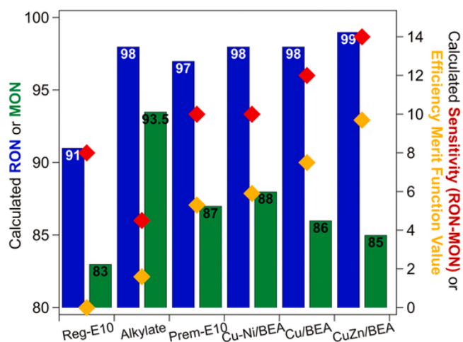
Fig. 7. Estimated fuel properties and expected engine efficiency for the C 5-8 hydrocarbon products (RON, MON, S, and efficiency merit) over BEA catalysts compared to U.S. Regular-E10, Premium-E10 gasolines [19] and a representative refinery alkylate stream [40] (“Alkylate”). Data for BEA catalysts reported at TON = 52 ± 2 mol C mol H+ -1 .
