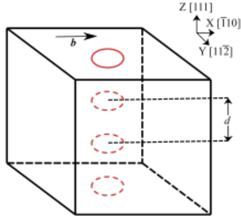
FIG. 8. Schematic of the simulation setup with multiple dislocation loops initiated on parallel glide planes. d and b represent the interloop spacing and Burgers vector, respectively.
