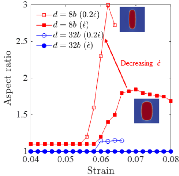
FIG. 7. Evolution of the aspect ratio of a dislocation loop within an array with respect to strain at low (open symbols) and high (solid symbols) strain rates. Lower strain rate loading leads to longer edge segments. The loops have an initial radius of r = 10b and the interloop spacing is 8b (red) and 32b (blue).
