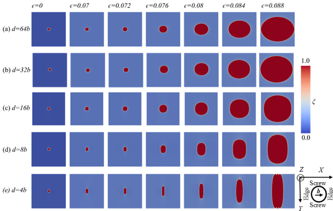
FIG. 1. The growth of one dislocation loop within an array under increasing applied strain. The dislocation loop has an initial radius of r = 5b . The interloop spacing d varies between 4b and 64b , significantly affecting the morphology of the dislocation loop as it expands. The loop lies on the X-Y plane, and the segment of the dislocation loop that is perpendicular (parallel) to the vector \mathbf{b} represents the pure edge (pure screw) segment. Schematics of the pure edge (and pure screw) segments of a dislocation loop and Burger's vector with reference to the coordinate system are provided on the lower right corner of the panel.
