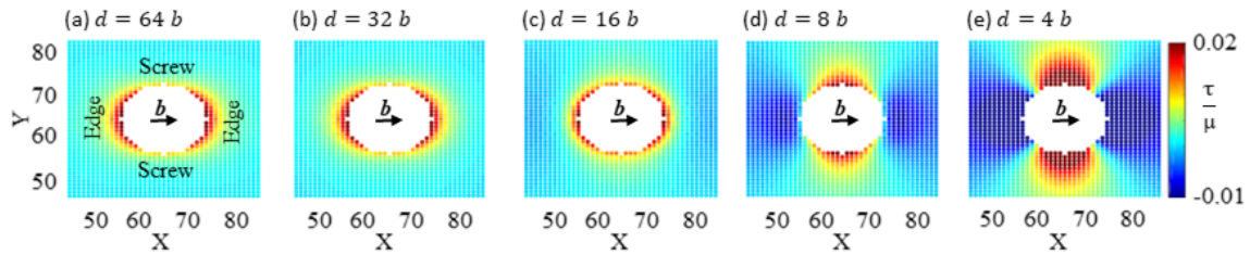
FIG. 2. The contour plot of the normalized shear stress \tau = \sigma_{xz} around the dislocation loop with r = 5b at zero strain predicted by the PFDD simulations. The stress inside the loop is removed for clarity. In Fig. 2a pure edge (perpendicular to Burger’s vector \mathbf{b} ) and pure screw (parallel to \mathbf{b} ) segments of the dislocation loop are shown.
