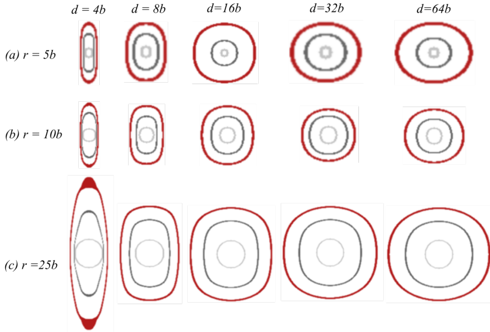
FIG. 4. Growth of a dislocation loop within an array where the initial dislocation loop has a radius of (a) r = 5b , (b) 10b , or (c) 25b . The interloop spacing d varies between 64b and 4b . Light gray, gray, and red colored loops represent the loop configurations at the initial (at \epsilon = 0 ), intermediate (at \epsilon \approx 0.038 ), and final (at \epsilon = 0.076 ) strain, respectively.
