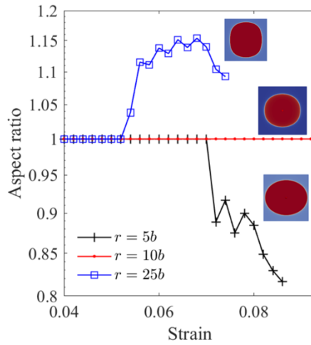
FIG. 5. The evolution of the aspect ratio of a dislocation loop within an array over time under increasing applied strain with an initial radius of r = 5b , 10b , or 25b , and a loop spacing of d = 32b . The aspect ratio is defined as the major axis over the minor axis, where the major axis is taken as the spacing between the screw segments of the loop.
