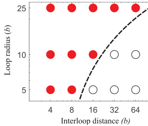
FIG. 6. Diagram showing the transition of a strong pinning effect between dislocation loops to a weak/negligible pinning effect as a function of the loop radius and interloop spacing. A filled red circle indicates pinning of the edge segments was observed, and an open black circle indicates no-pinning effect was observed.
