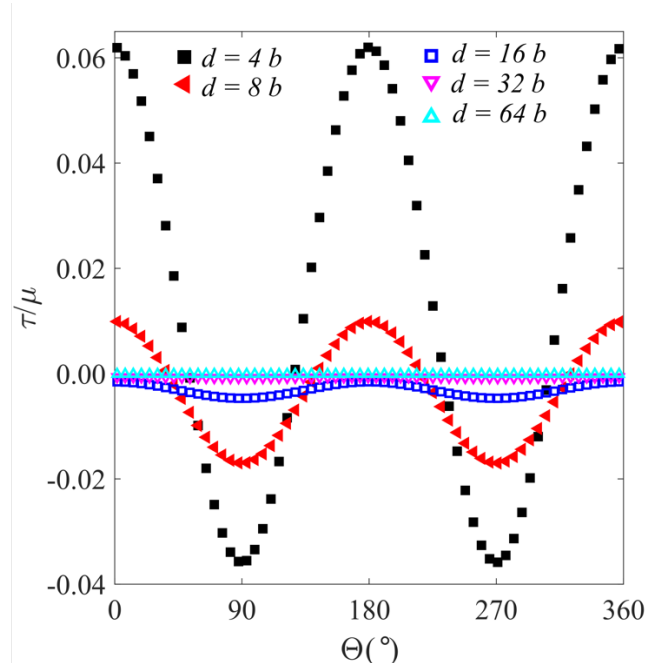
FIG. 3. The distribution of the shear stress \tau_{inter} around the dislocation loop at zero applied strain calculated with the superposed analytical solution describing the stress caused by elastic interactions between loops.
