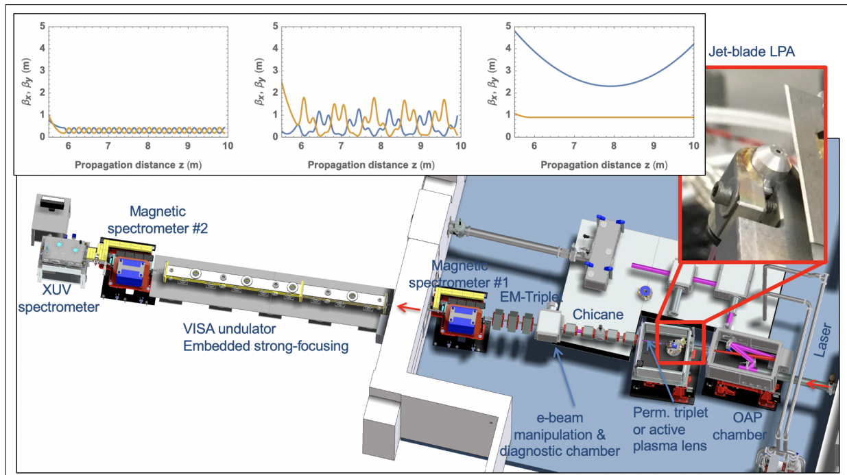
Figure 7: Schematic layout of the BELLA Center's Laser-Plasma Accelerator FEL beamline. The inset show the electron beam beta function (beam size squared) inside the undulator in the (left) optimally-matched strong-focusing undulator, (middle) a mismatched strong-focusing undulator, and (right) an optimized natural-focusing undulator. The strong-focusing undulator allows for higher beam density over the full undulator length.
