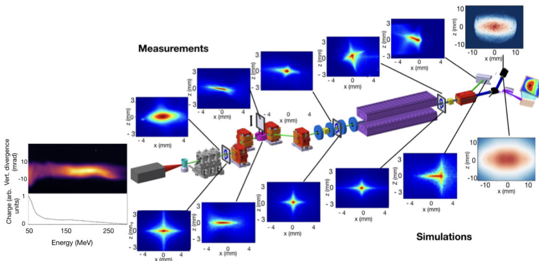
Figure 2: COXINEL electron and photon beam measurements compared to simulations. Left : electron beam spectrometer measurements and transverse distributions along the screens (up : measurements, down : simulations using the measured electron beam distribution as an input). Right : undulator radiation transverse pattern (measured with a CCD camera and modeled using the transported electron beam without electron energy selection).
