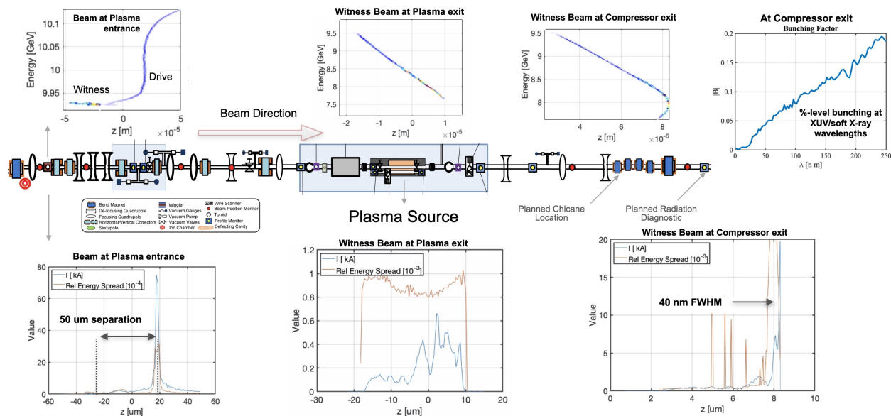
Figure 1: Schematic of the FACET-II Experimental area with the planned location of an additional small chicane and radiation diagnostic to be used for XFEL experiments. The simulated longitudinal phase space evolution shows the compression of the electron beam to attosecond duration with %-level bunching at XUV/soft X-ray wavelengths.
