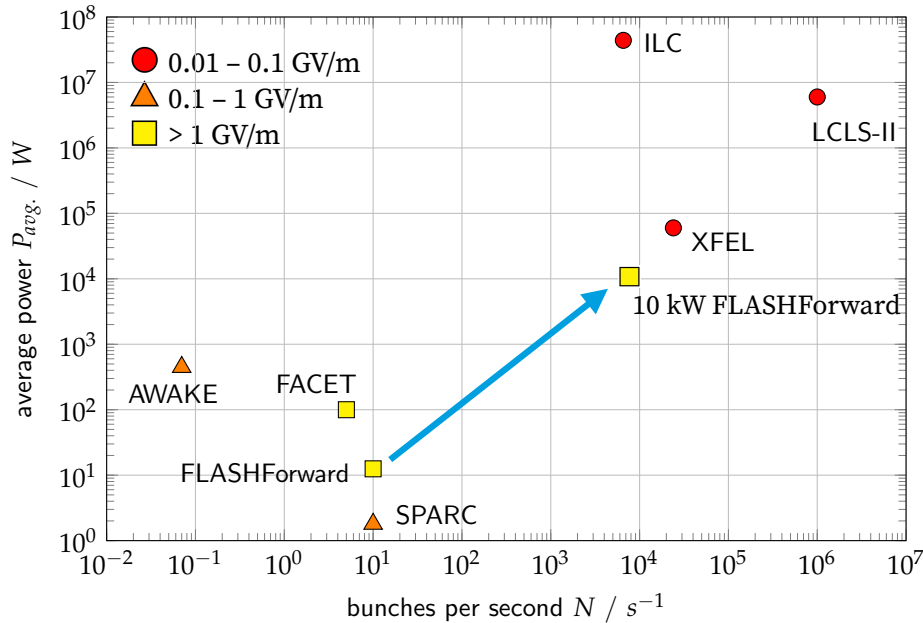
Figure 3: Average power as a function of the number of drive bunches per second at a range of existing or planned a) plasma-wakefield research facilities (bottom left corner), and b) photon-science and high-energy-physics user facilities (top right). The blue arrow represents the leap towards a beam-driven plasma-based FEL by using high-average-power upgrades to FLASHForward as a gateway.
