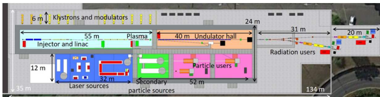
Figure 8: Layout of the EuPRAXIA@SPARC_LAB infrastructure.
