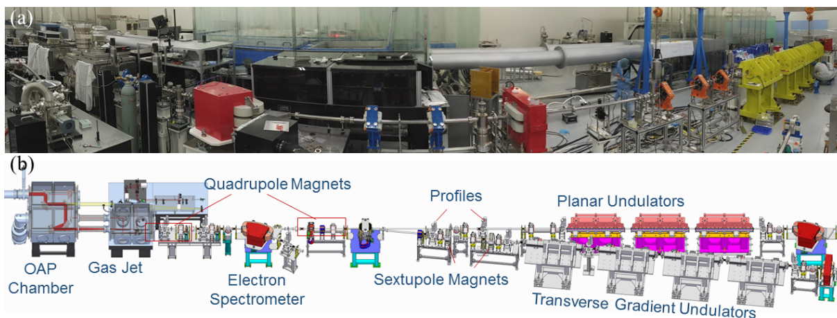
Figure 5: The SIOM-FEL setup with planar undulators and transverse gradient undulators.
