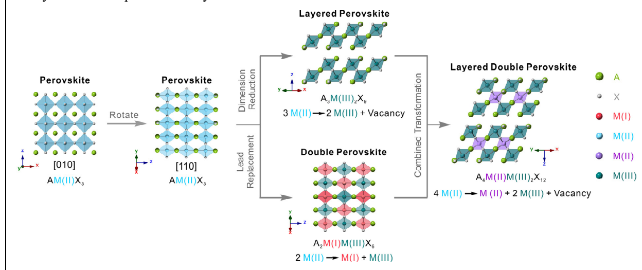
Scheme 1. Schematic of the evolution of metal halide perovskites from the conventional 3D perovskite to layered double perovskite crystal structure.
