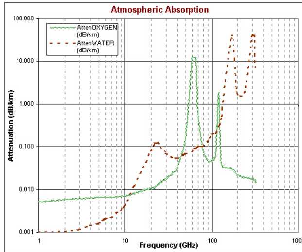
Fig. 2. Attenuation values of oxygen and water [6].
