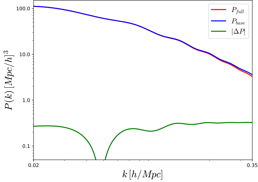
FIG. 1. Shown here are the full power spectrum (red) of Eq. 16, the base model (blue) from [39], and the absolute value of the difference between them (green). \Delta P changed sign from positive at small k to negative at k \gtrsim 0.04 h/\text{Mpc} . Both here and in Figure 2 we took c_1 and c_2 from [39] and the remaining c coefficients from FGPA. These were evaluated at \mu = 1/\sqrt{3} .
