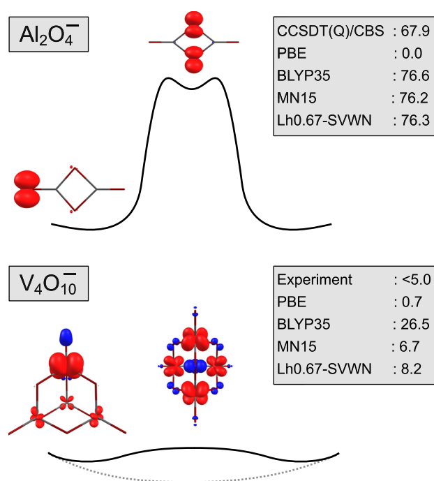
FIG. 5. Spin-density distributions ( \pm 0.01 a.u. isosurfaces) of Al_2O_4^- and V_4O_{10}^- at minimum structures (left) and a transition state/high-lying minimum (right) calculated at the \omega B97X-D 169 /def2-TZVP level. Relative energies at different levels of theory are given in kJ/mol. CBS denotes the complete basis set limit. The drawings give a qualitative impression of the potential energy curves (dashed line for a delocalized structure). The D_{2d} structure of the V_4O_{10}^- transition state was deduced from the experimental spectra (see Ref. 166 for details). Reprinted (adapted) with permission from Klawohn et al. , J. Chem. Theory Comput. 14, 3512–3523 (2018). Copyright 2018 American Chemical Society.
