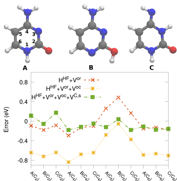
FIG. 17. (Top) Tautomers of cytosine considered in this study. The following color scheme was used for the atoms: H (white), C (gray), N (blue), and O (red). (Bottom) Errors in d -GKS-spRPA based C(1s) CEBEs for cytosine tautomers compared to CVS-ADC(4) values. 264 HF exchange is denoted as HF. For the d -GKS-spRPA calculations, def2-TZVPP basis sets and the PBE potential (grid size m5) were used. The molecular geometries were optimized using the PBE energy functional. Reprinted with permission from Voora et al. , J. Chem. Phys. 151 , 134106 (2019). Copyright 2019 AIP Publishing LLC.
