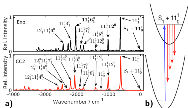
FIG. 26. (a) Single vibronic level (SVL) fluorescence spectrum of anthracene excited to the S_1+11 vibronic level (black: experimental, 296 red: calculated using the radless module). (b) Schematic representation of the SVL process; upon excitation to the S_1+11 level (blue arrow), emission to the various vibrational levels in the ground state occurs (red arrows). Reprinted (adapted) with permission from Tapavicza, J. Phys. Chem. Lett. 10 , 6003–6009 (2019). Copyright 2019 American Chemical Society.
