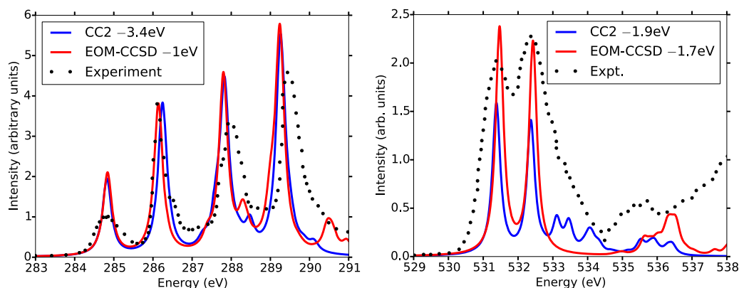
FIG. 13. Comparison of the fc-CVS-CC2 and fc-CVS-EOM-CCSD NEXAFS spectra at the carbon and oxygen K-edges in uracil. Basis set 6-311++G**. 246,247 The CCSD results are from Ref. 244. Experimental spectra have been re-digitized from Ref. 245.
