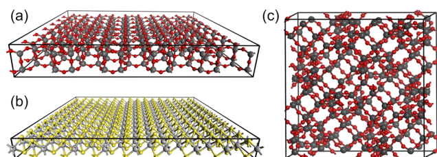
FIG. 9. Benchmark systems with 2D and 3D periodicity: (a) 5 \times 7 unit cell of 2D \text{SiO}_2 , 213 (b) 8 \times 12 unit cell of 2D \text{MoS}_2 , and (c) unit cell of 3D faujasite zeolite (FAU) (O, red; S, yellow; Si, dark gray; and Mo, light gray).
