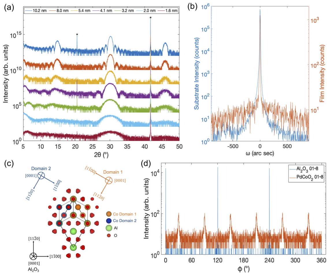
FIG. 3. X-ray diffraction (a) \theta - \theta scans of samples A-G showing only 000 \ell reflections of \text{PdCoO}_2 and Laue oscillations indicating an abrupt and smooth film-substrate interface. Asterisks (*) denote substrate reflections. The scans are vertically offset from each other for clarity. (b) Overlaid rocking curves in \omega of the 0006 film and substrate reflections of sample B; the comparable widths (9 arc sec for both the substrate and film) indicate low out-of-plane mosaicity. (c) In-plane epitaxial relationship between (0001) \text{PdCoO}_2 and (0001) \text{Al}_2\text{O}_3 showing the two \text{PdCoO}_2 domains with equivalent lattice mismatch with respect to \text{Al}_2\text{O}_3 and (d) off-axis \phi scan of 01·8 reflections of \text{PdCoO}_2 and \text{Al}_2\text{O}_3 of sample A showing three poles for the substrate, but six poles for the film due to 180^\circ in-plane rotation twinning.
