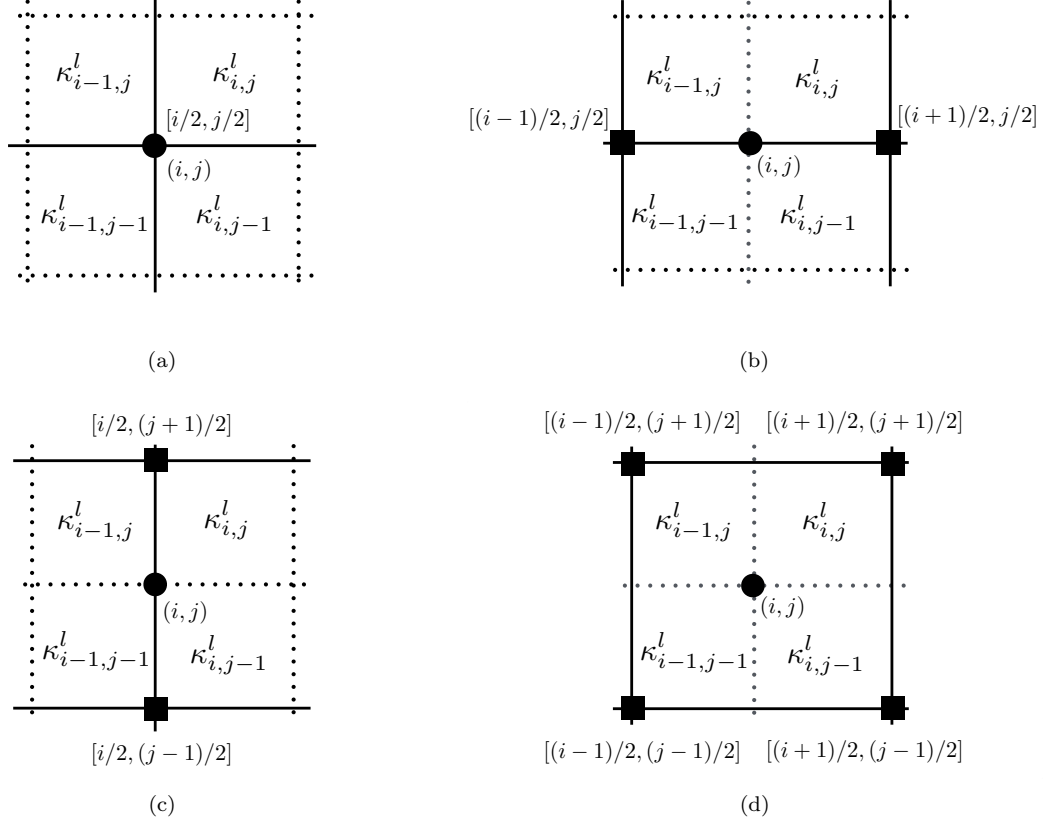
Figure 5: The image-based inter-grid operator scheme. The solid lines (—) denote the coarse grid. The dotted lines (⋯⋯) denote the fine grid. The circle (●) marks the nodal value to be prolonged, whose indexes are denoted using (\cdot, \cdot) . The square (■) marks the nodal value known from the coarse grid, whose indexes are denoted using [\cdot, \cdot] . The \kappa_{i,j}^l is the element-wise material property acquired from the l th SVB-LOD microstructure (see Eq. (3)).
