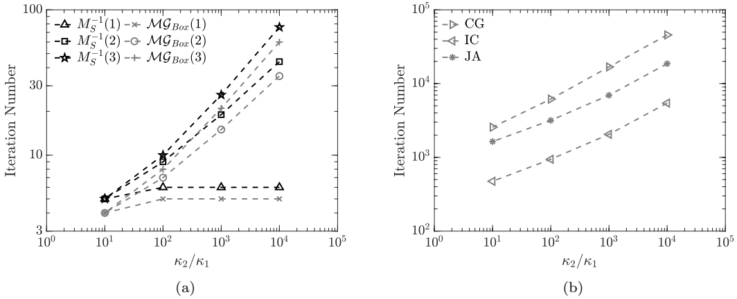
Figure 13: The number of iterations required to converge to the solution using different preconditioners. The results are shown for a varying coefficient contrast. (a) The M_S^{-1}(L) and MG_{Box}(L) preconditioners with L \in \{1, 2, 3\} . (b) The IC, JA preconditioners and CG. The number of iterations are also listed in Table 5.
