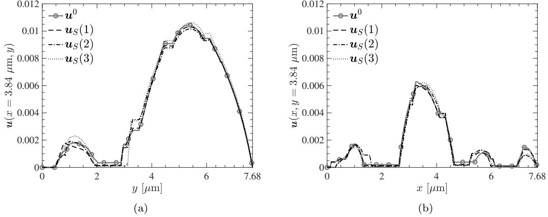
Figure 16: The comparison between the fine grid solution and solutions from the IROM. The coefficient contrast is \kappa_2/\kappa_1 = 10000 . (a) x = 3.84 \mu\text{m} . (b) y = 3.84 \mu\text{m} .
