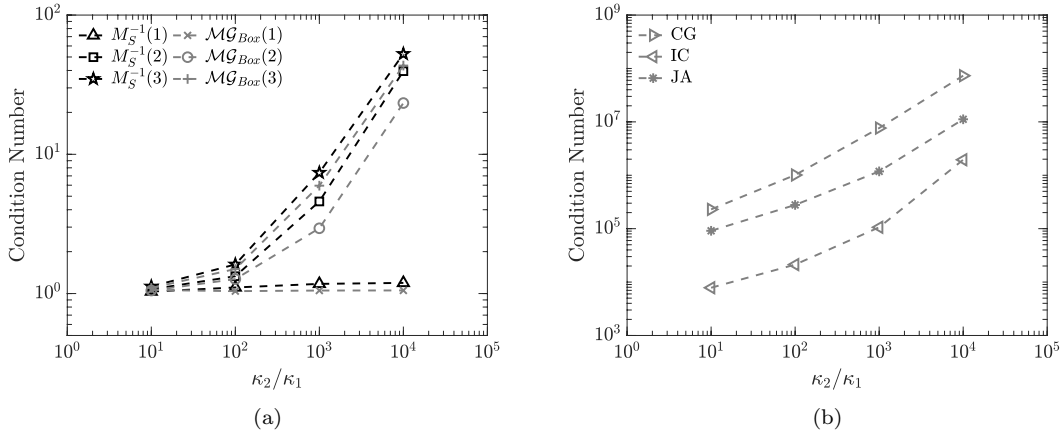
Figure 12: The condition number of the coefficient matrix before and after preconditioning with varying coefficient contrasts. (a) The M_S^{-1}(L) and MG_{Box}(L) preconditioners with L \in \{1, 2, 3\} . (b) The IC, JA preconditioners and CG. The condition numbers are also listed in Table 5.
