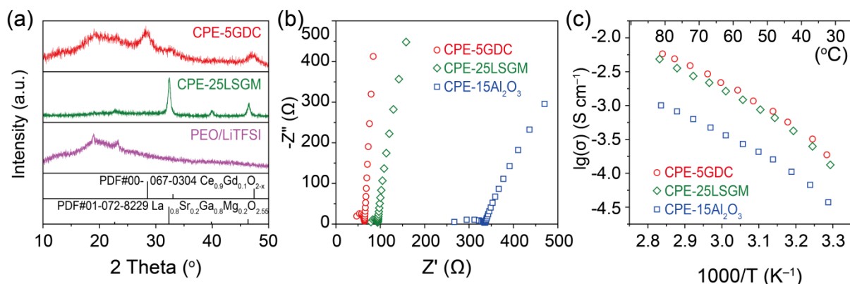
Figure 1. (a) XRD patterns, (b) impedance plots (30 °C), and (c) Arrhenius plots of \text{Li}^+ conductivities of the composite electrolytes ([EO]/[Li] ratio n = 10 ).
