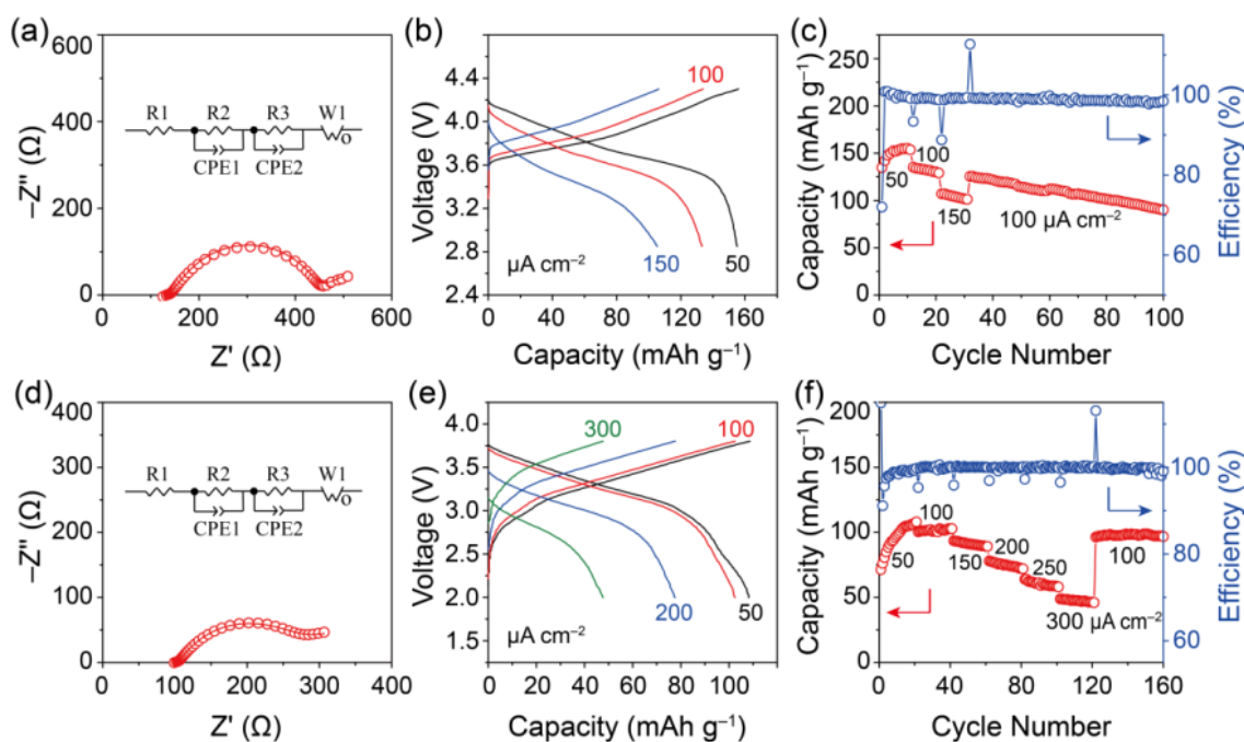
Figure 5. All-solid-state Li/NMC cell cycled at 35 °C. (a) Electrochemical impedance plots, (b) charge/discharge voltage profiles, and (c) capacity retention and cycling efficiency. All-solid-state Li/polyaniline cells cycled at 35 °C. (d) Electrochemical impedance plots, (e) charge/discharge voltage profiles, and (f) capacity retention and cycling efficiency. (The area of the cathodes and Li metal were 0.3 and 0.5 cm 2 , respectively.)
