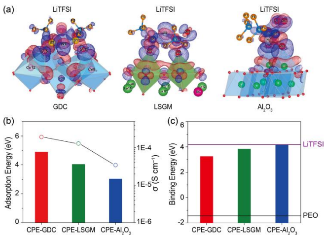
Figure 3. (a) Calculated differential electron density distribution on the surface of GDC, LSGM, and \text{Al}_2\text{O}_3 . Blue and red isosurface represent electron accumulation and depletion, respectively. (b) TFSI ^- adsorption energy on the surface of the crystal and the corresponding experimental measured \text{Li}^+ conductivity. (c) Calculated Li binding energy of the TFSI ^- adsorbed on each substrate surface, free TFSI ^- (purple), and free PEO (black).
