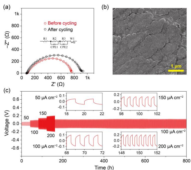
Figure 4. The symmetric Li/Li cell with CPE–5GDC composite electrolyte. (a) The impedance plots of the Li/Li symmetric cell before and after cycling. (b) SEM image of lithium metal surface after cycling. (c) The cycling performance of the symmetric Li/Li cell with different current densities at 35 ^\circ\text{C} . The surface area of Li metal was 0.5 \text{cm}^2 .
