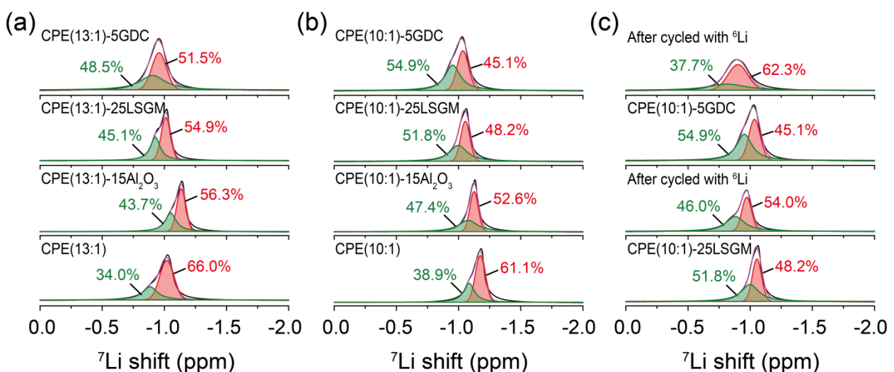
Figure 2. ^7\text{Li} MAS NMR spectra of the composite electrolytes with different [EO]/[Li] ratios (a) n = 13 , (b) n = 10 ; (c) ^7\text{Li} MAS NMR spectra of the composite electrolyte before/after ^6\text{Li} \rightarrow ^7\text{Li} tracer-exchange experiment at room temperature.
