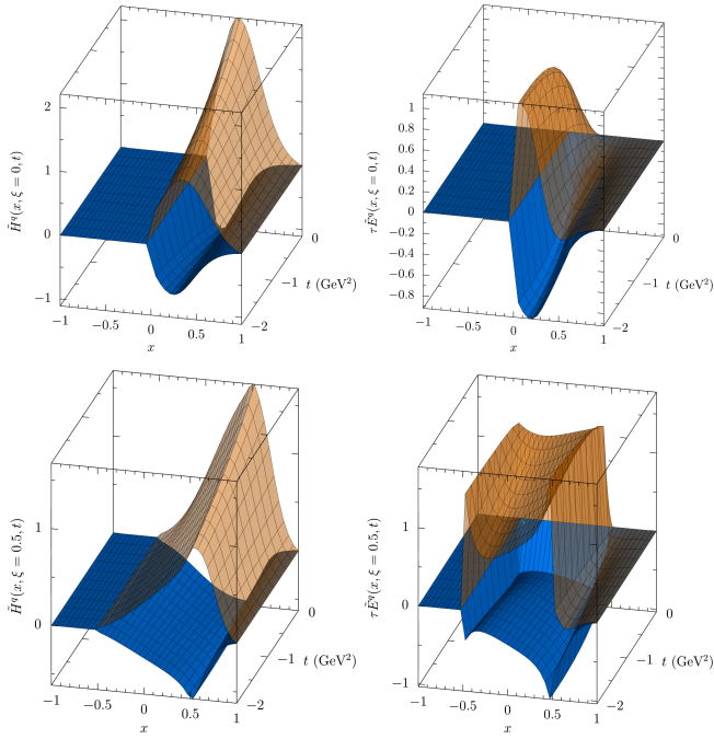
FIG. 2. The helicity-dependent proton GPDs at the model scale of Q^2 = 0.16 \text{ GeV}^2 , where the GPD \tilde{E}^q(x, \xi, t) has been scaled by a factor \tau = -t/(4M_N^2) . The top row is for \xi = 0 and the bottom row has \xi = 0.5 . The transparent (orange) surface is up quarks and the opaque (blue) surface is down quarks.
