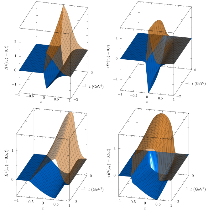
FIG. 3. The helicity-dependent proton GPDs at the scale of Q^2 = 4.0 \text{ GeV}^2 , where the GPD \tilde{E}^q(x, \xi, t) has been scaled by a factor \tau = -t/(4M_N^2) . The top row is for \xi = 0 and the bottom row has \xi = 0.5 . The transparent (orange) surface is up quarks and the opaque (blue) surface is down quarks.
