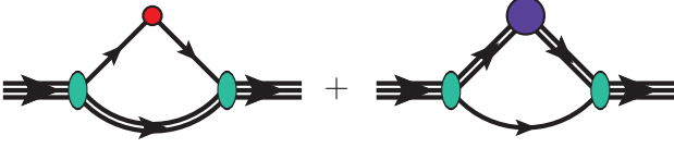
FIG. 1. Diagrams contributing to the leading-twist proton GPDs. On the left is the quark diagram and on the right is the diquark diagram. The single line is the dressed quark propagator, the double line the diquark propagator, the shaded oval the Faddeev vertex, and the shaded circles represent the dressed quark and diquark GPDs.
