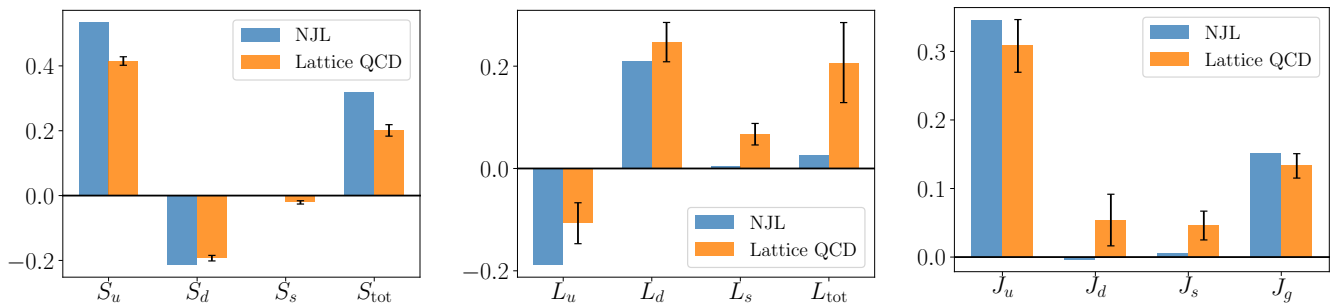
FIG. 5. Comparison of NJL model spin decomposition to the lattice QCD results of Ref. [41] at Q^2 = 4 \text{ GeV}^2 . The NJL results contain contributions from both scalar and axial vector diquarks.
