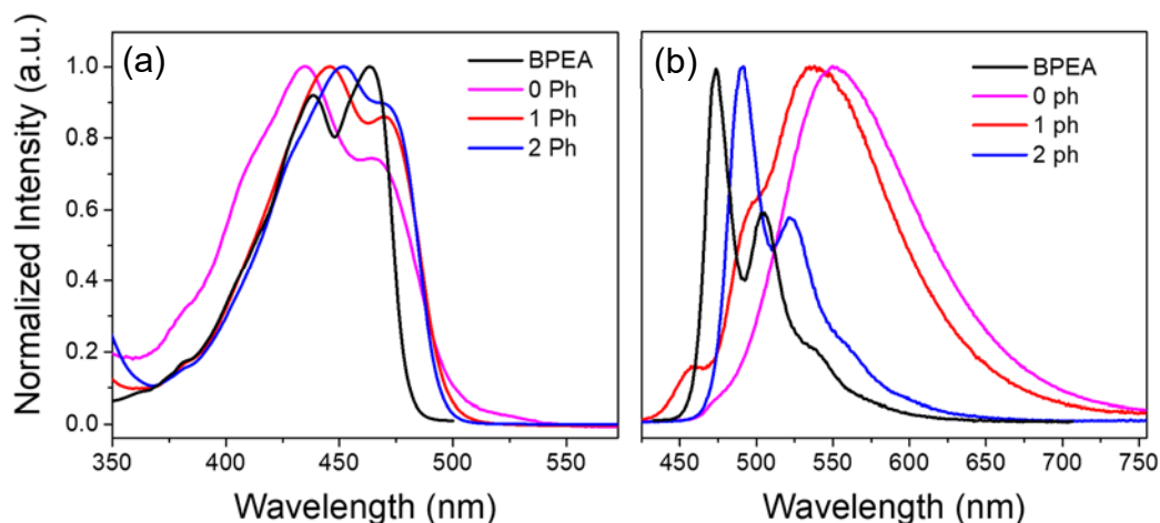
Figure 1. (a) Steady state absorbance and (b) emission spectra of BPEA monomer and dimers in DCM.
