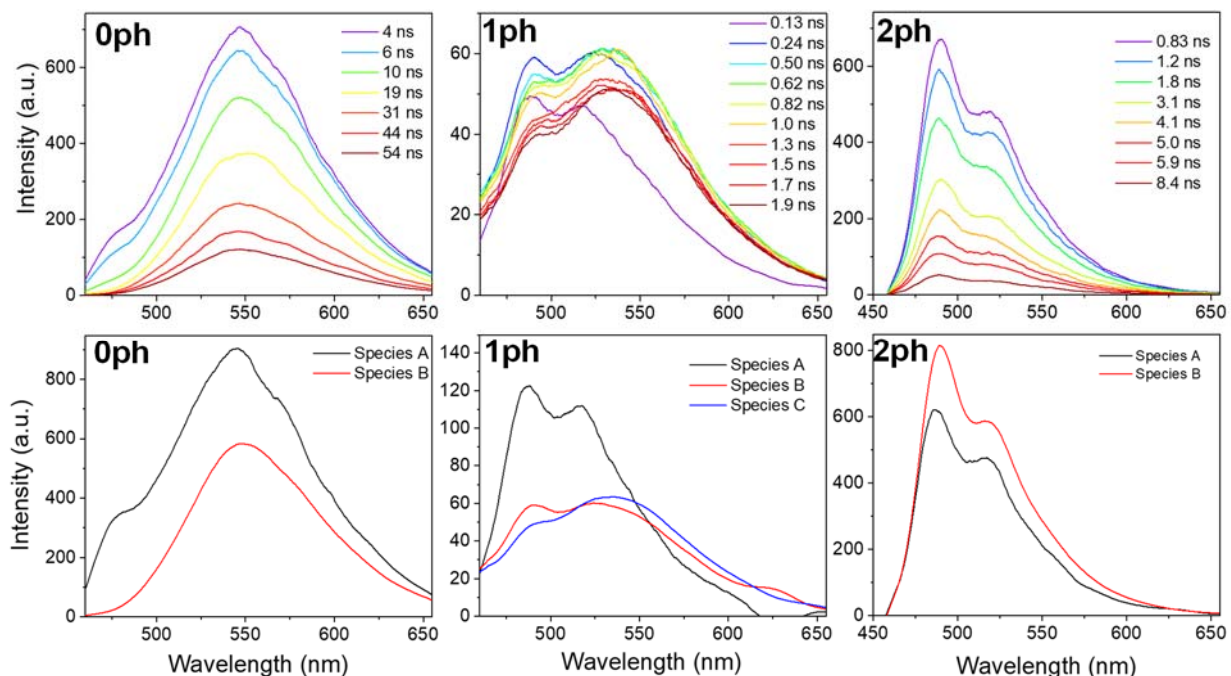
Figure 2. TRF spectra of BPEA dimers in DCM upon photoexcitation at \lambda_{\text{ex}} = 414\text{nm} (15 nJ/pulse). The TRF spectra are globally fit using an, A \rightarrow B \rightarrow C \rightarrow \text{GS} , evolution-associated decay model and the resulting spectral fits are shown in the bottom panel. Additional time windows, wavelength fits and population vs. time fits are shown in Figure S3-S12.
