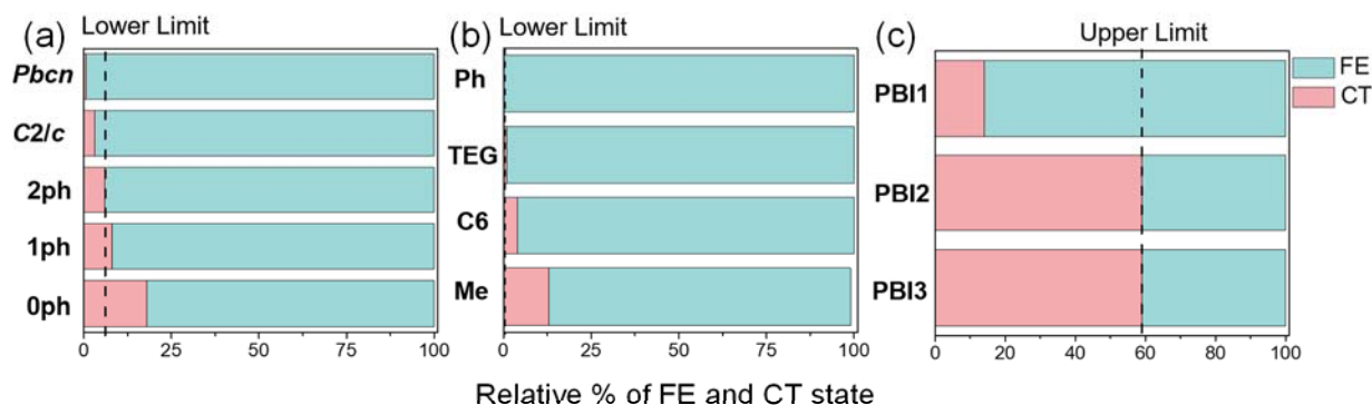
Figure 5. Calculated percent contribution of FE and CT states. The lower limit of the CT contribution for excimer formation is shown as a dashed line for the (a) BPEA and (b) DPP systems and the upper limit is shown for the (c) PDI systems. The calculated FE and CT contributions are shown in Table S21.
