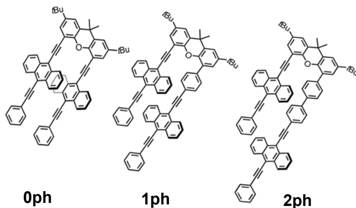
Scheme 1. BPEA covalent dimers: 0ph , 1ph , and 2ph .
