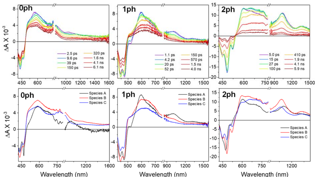
Figure 3. fsTA spectra of BPEA dimers in DCM upon photoexcitation at \lambda_{\text{ex}} = 414\text{nm} ( 1 \mu\text{J/pulse} ). The fsTA spectra are globally fit using A \rightarrow B \rightarrow C \rightarrow GS kinetic model and the resulting spectral fits are shown in the bottom panel. Wavelength fits and population vs. time fits are shown in Figures S13-S23.
