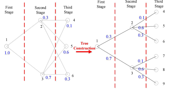
Fig. 2. A scenario tree.
